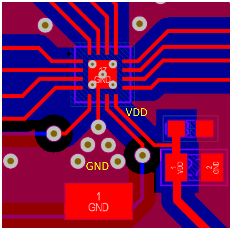
图 9-13. Recommended Layout
