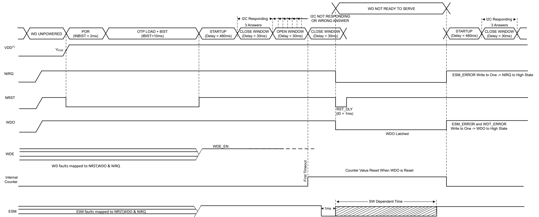
图 7-17. TPS389C03 ESM Error After WD Time-out
