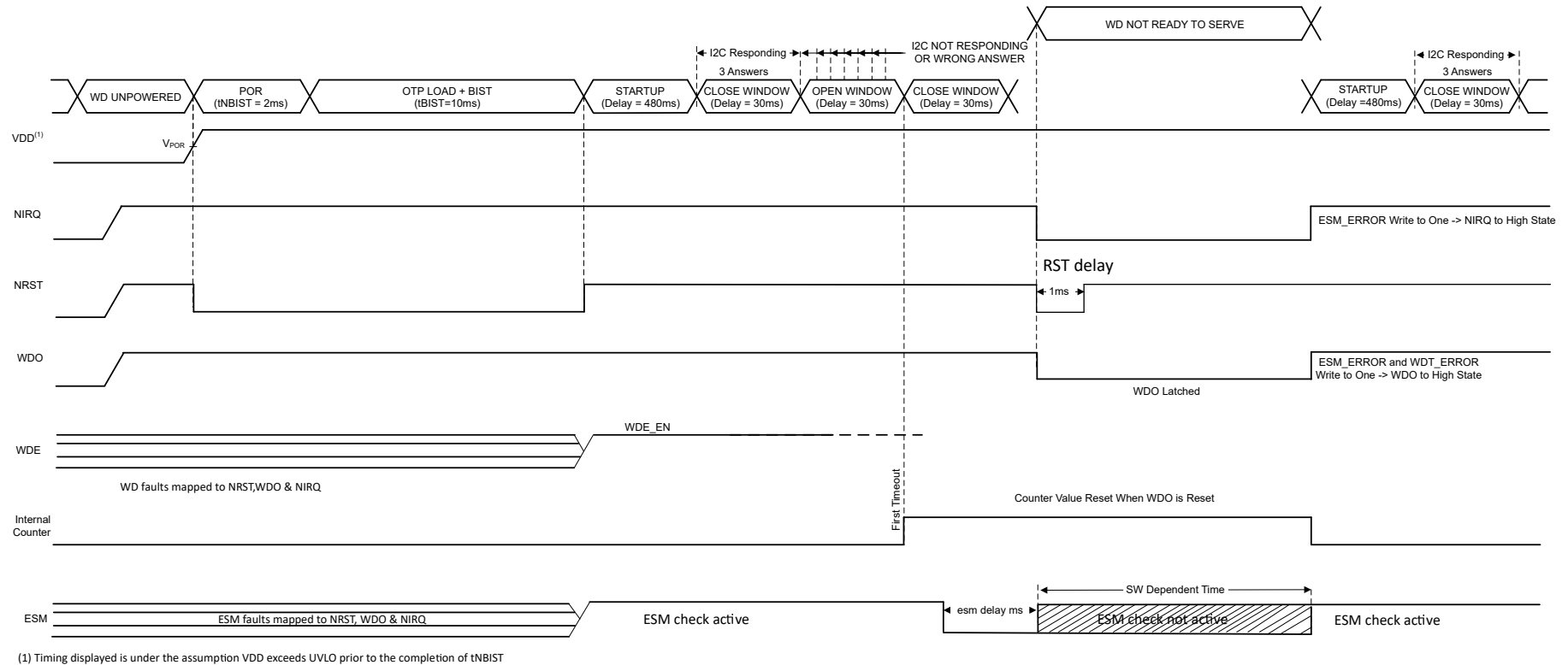
图 7-24. WD Error Followed by ESM Fault (WD Enabled)
