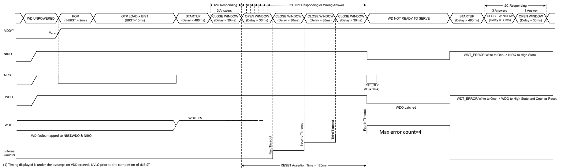
图 7-15. TPS389C03 OPEN Window Error WDO Latched
