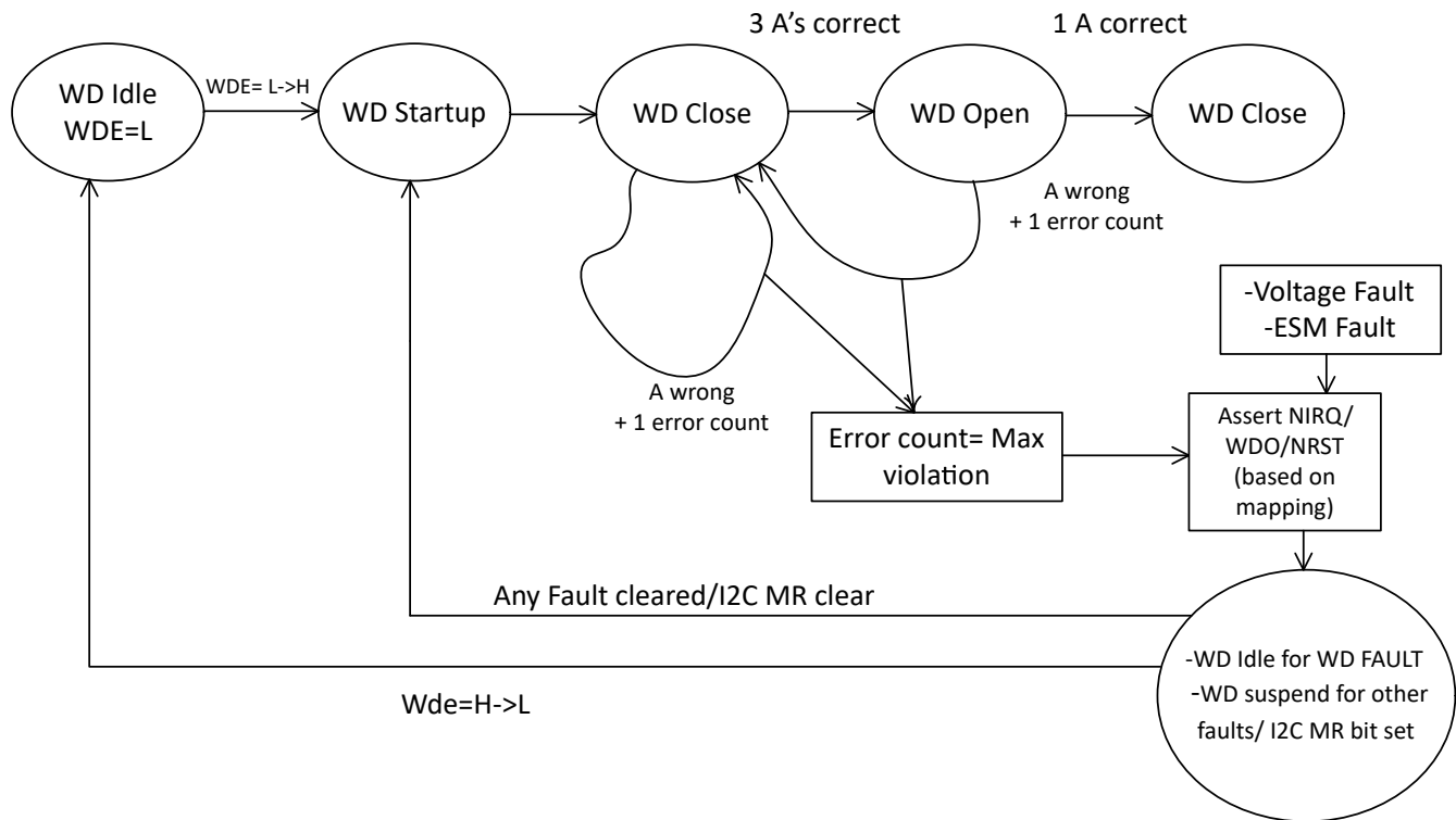
图 7-20. Q&amp;A Watchdog State Diagram
