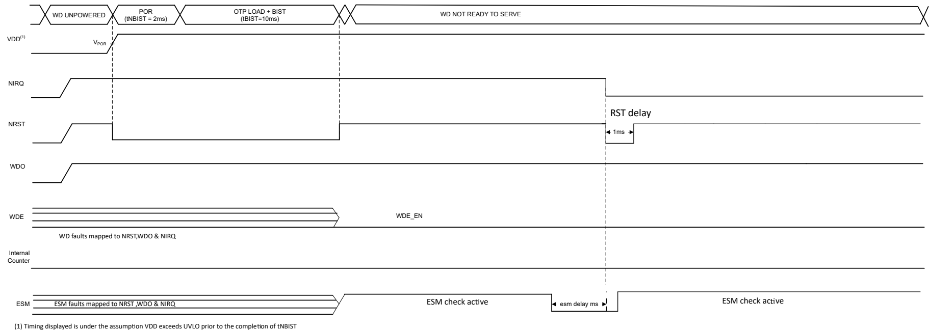
图 7-26. Transient ESM Fault (WD Disabled)
