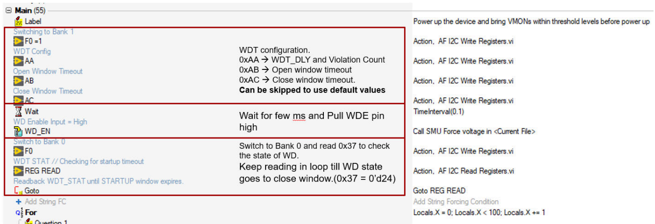
图 7-21. Q&amp;A Watchdog Test Program Page 1
