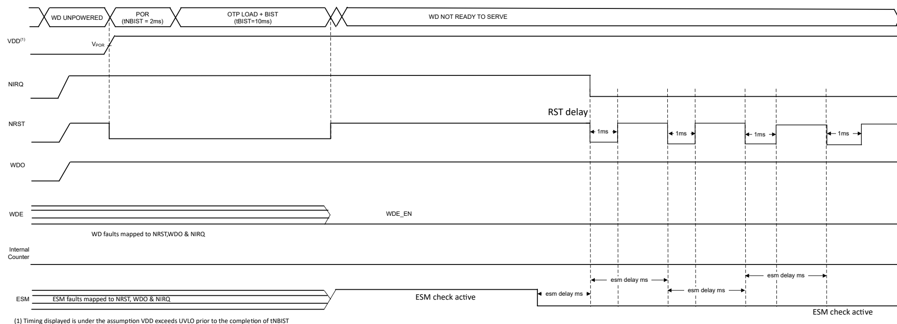
图 7-27. Permanent ESM Fault (WD Disabled)
