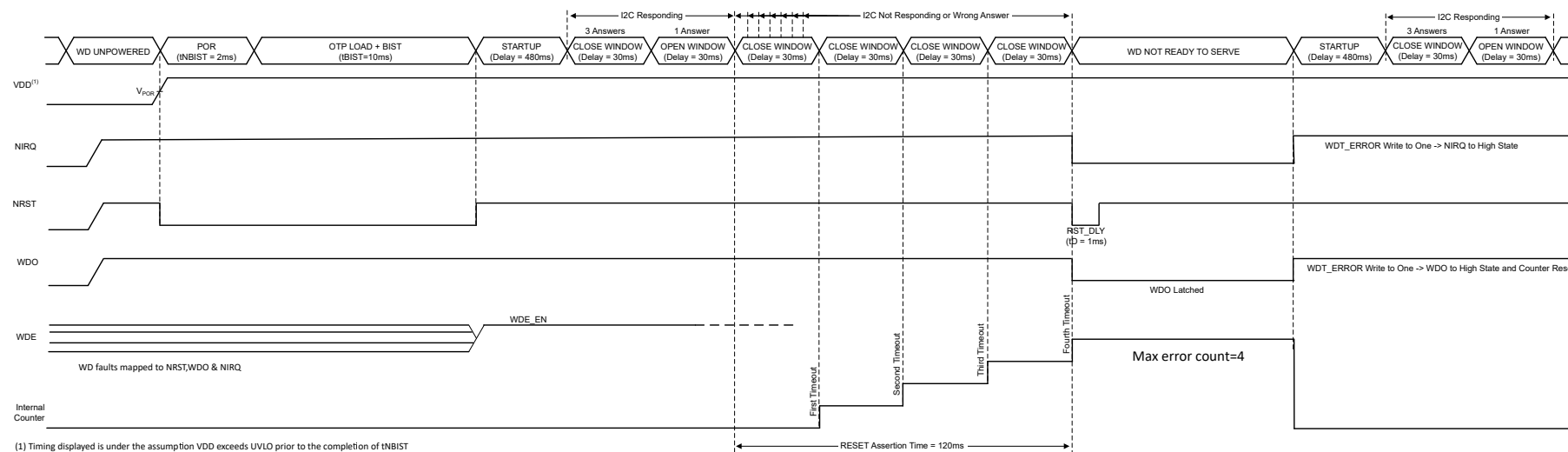
图 7-12. TPS389C03 CLOSE Window Error WDO Latched
