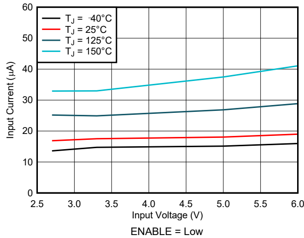
图 7-3. Quiescent Supply Current
