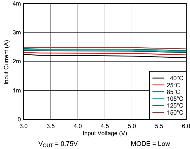
图 7-1. Operating Supply Current (Power Save Mode)
