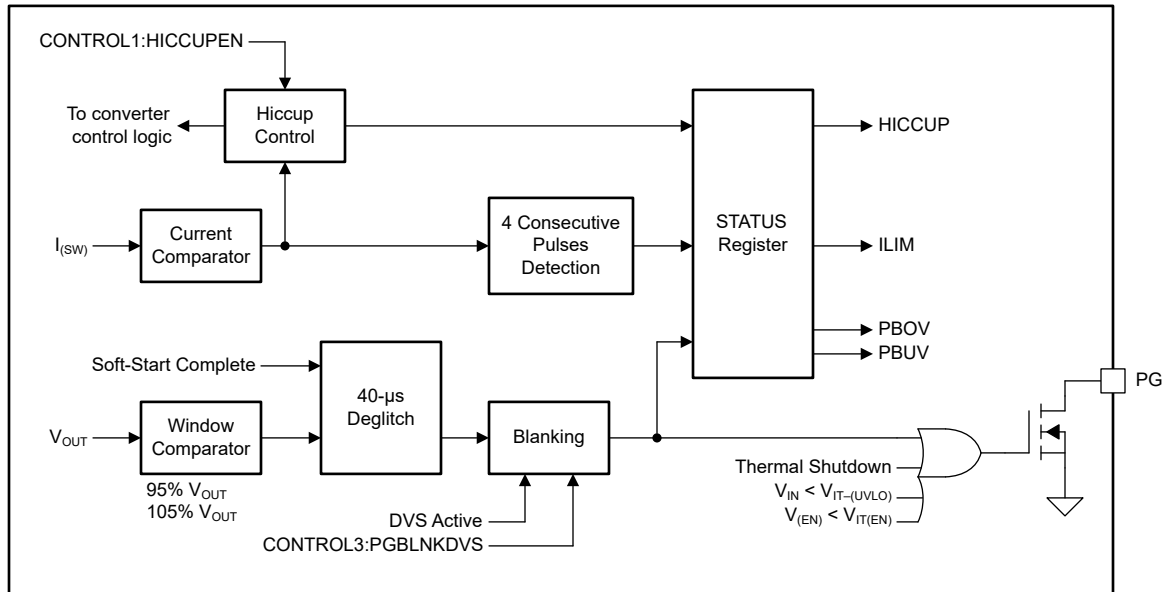
图 8-12. Power-Good Functional Block Diagram (Standalone or Primary Device)
