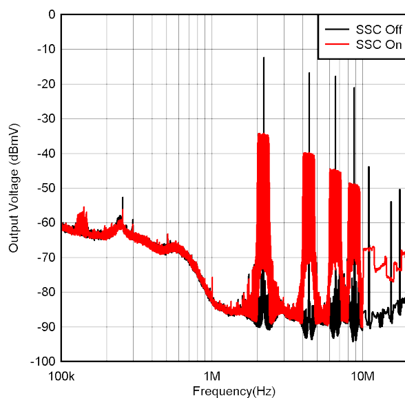
图 10-19. Spread Spectrum Operation
