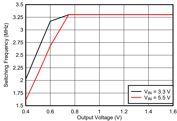
图 7-5. Maximum Switching Frequency vs V_{IN} and V_{OUT}
