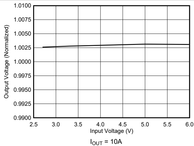
图 10-12. Line Regulation
