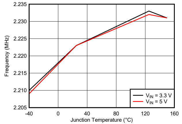
图 7-4. Switching Frequency vs Temperature
