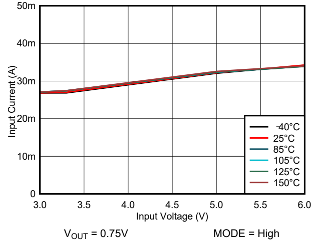
图 7-2. Operating Supply Current (Forced PWM)
