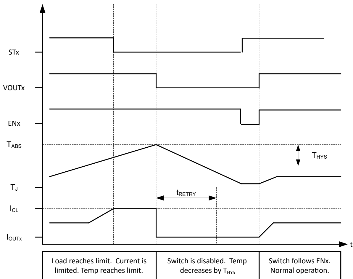
图 8-8. Thermal Shutdown - Latched Behavior
