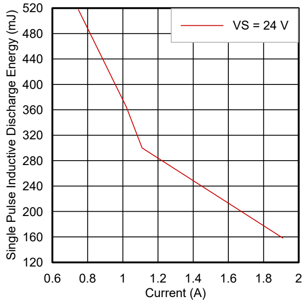
图 8-13. Maximum Energy Dissipation ( E_{AS} ) Allowed T_{J, START} = 125^{\circ}\text{C} - Single Pulse, One Channel
