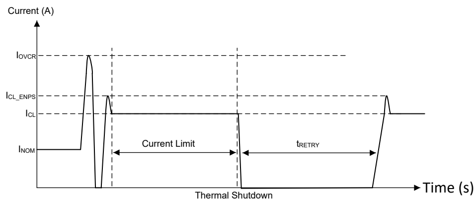
图 8-6. On-State Short-Circuit Behavior
