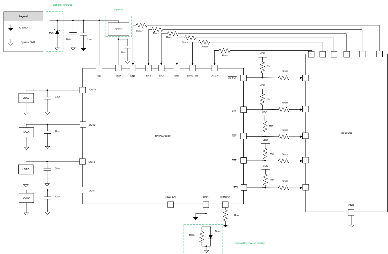
图 9-1. Typical Application Circuit
