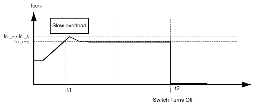
图 8-3. Overload Response
