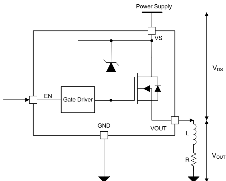
图 8-10. Driving Inductive Load
