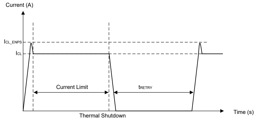
图 8-5. Enable into Short-Circuit Behavior
