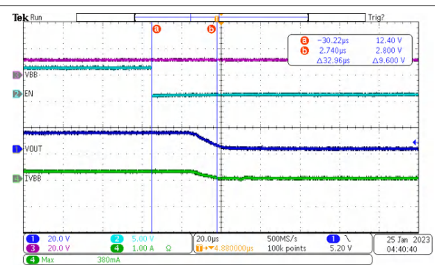
图 6-2. Turn-off Time (t OFF )
