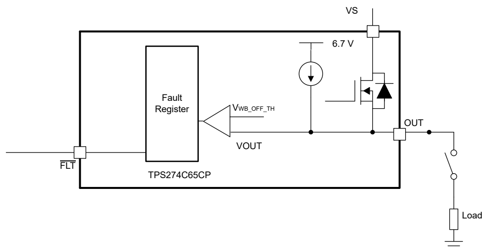
图 8-15. Open-Load Detection Circuit
