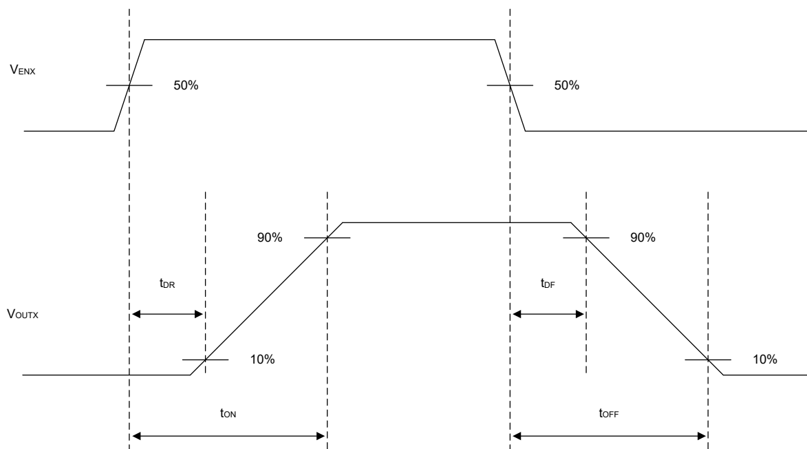
图 7-1. Switching Characteristics Definitions
