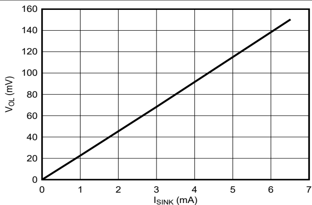
图 9-7. Open-Drain Active Low V_{OL} vs I_{RESET} ( V_{DD} = 2.7\text{V} )
