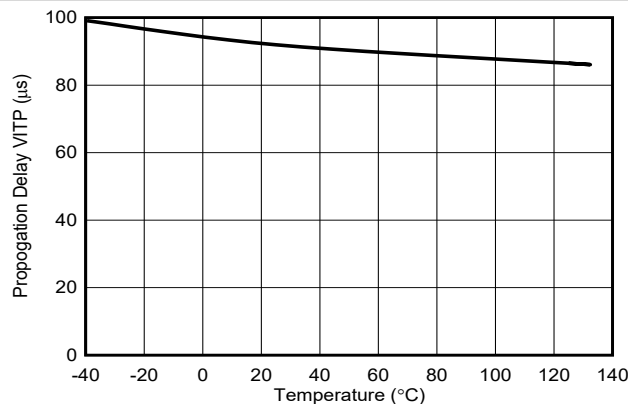
图 9-10. Propagation Delay (Overvoltage) vs Temperature ( V_{IT} = 0.8\text{V} , CTS = Enabled = 50pF)
