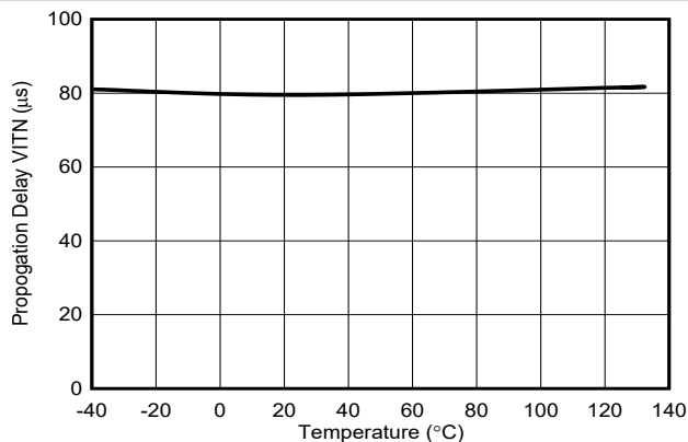
图 9-9. Propagation Delay (Undervoltage) vs Temperature ( V_{IT} = 0.8\text{V} , CTS = Enabled = 50pF)
