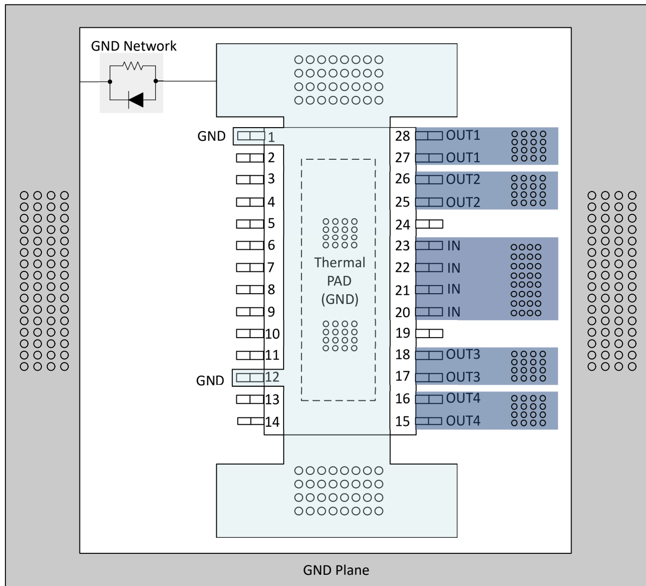
图 9-8. Layout Example With a GND Network
