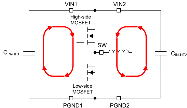
图 9-20. Input Current Loops
