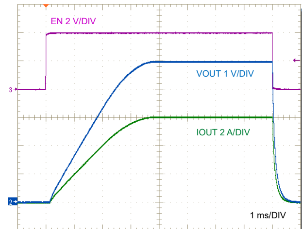
图 9-5. LM64460-Q1 Enable On and Off, 6-A Resistive Load
