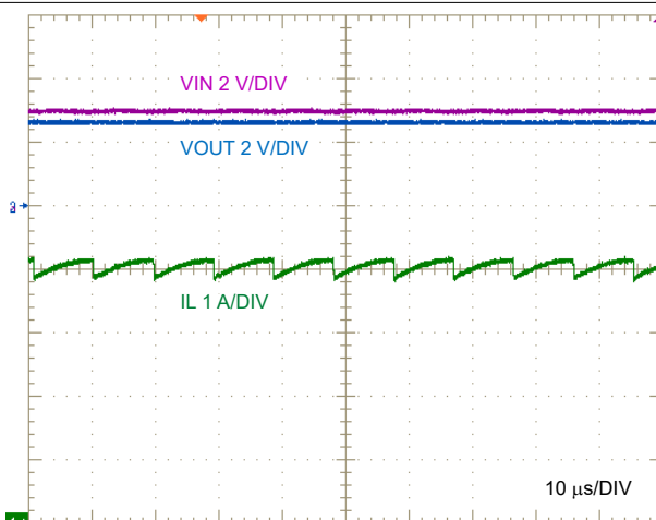
图 9-11. LM64460-Q1 Frequency Foldback in Dropout, V_{IN} = 3 \text{ V}
