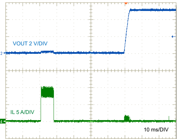
图 8-19. Short-Circuit Recovery
