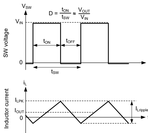
图 8-23. FPWM Mode Operation
