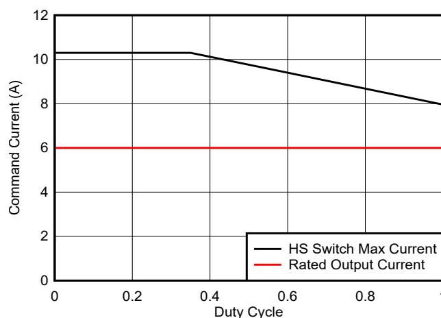
图 8-16. HS Switch Maximum Current as a Function of Duty Cycle for the LM64460-Q1
