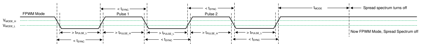
图 8-6. Spread Spectrum Disabled in FPWM Mode
