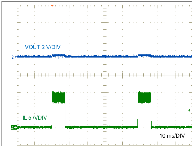
图 8-18. Inductor Current Bursts During Hiccup
