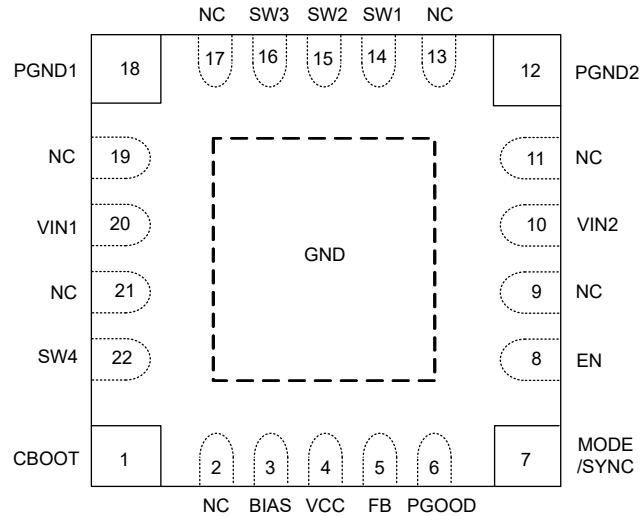
图 6-1. 22-Pin Enhanced HotRod™ QFN RYF Package (Top View)
