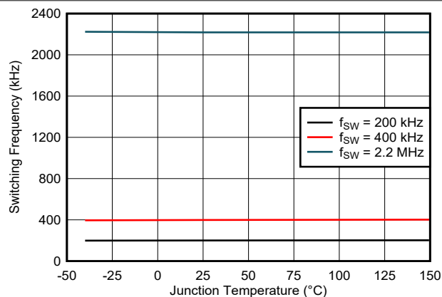
图 7-5. Switching Frequency Set by SYNC
