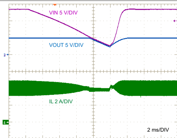
图 9-10. LM64460-Q1 Line Transient and Recovery from Dropout
