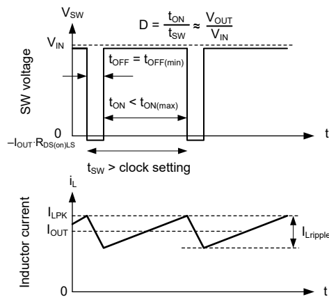
图 8-25. Switching Frequency and Output Voltage in Dropout
