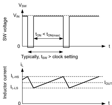
图 8-17. Current Limit Waveforms
