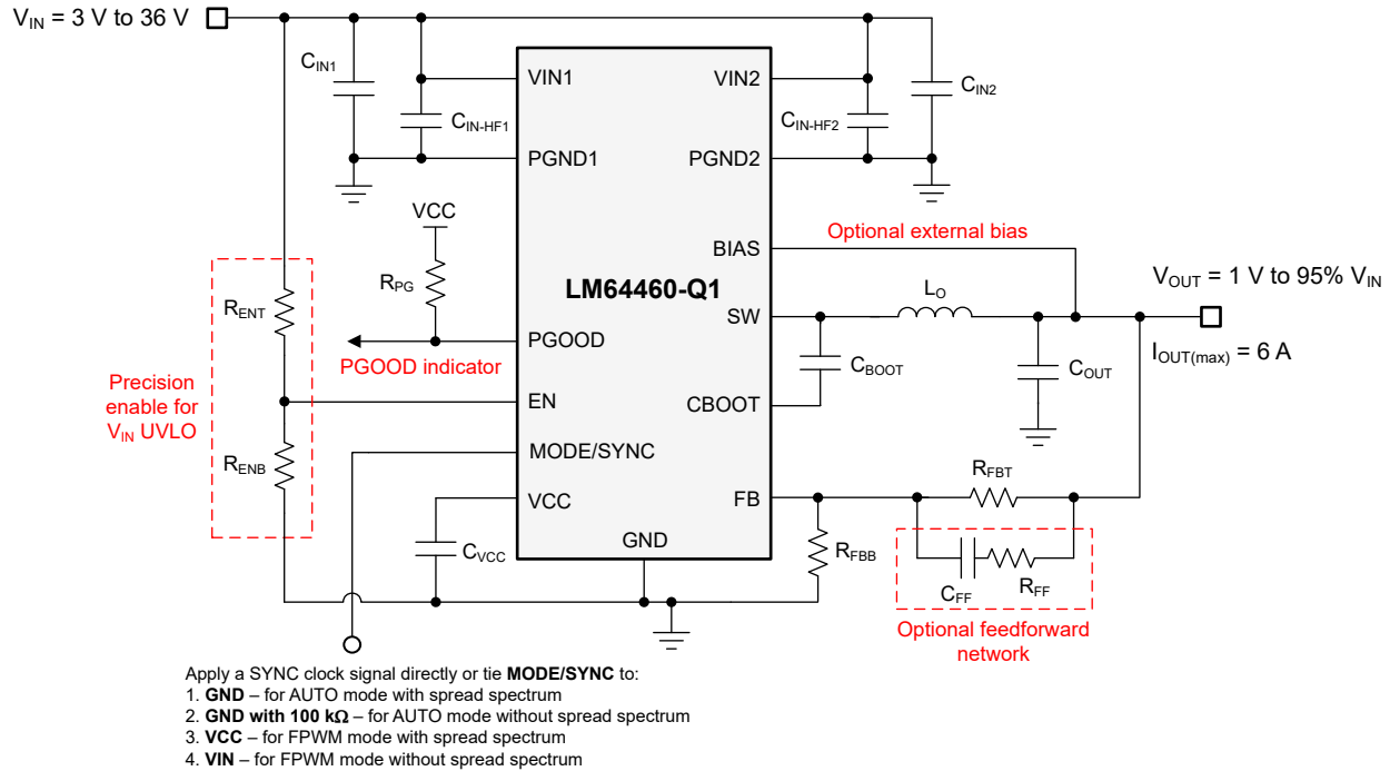
图 8-1. LM64460-Q1 Schematic Diagram with Input Voltage Operating Range of 3 V to 36 V
