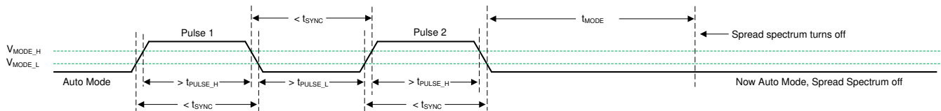
图 8-7. Spread Spectrum Disabled in AUTO Mode
