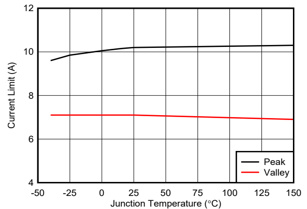
图 7-4. High-Side and Low-Side Current Limits
