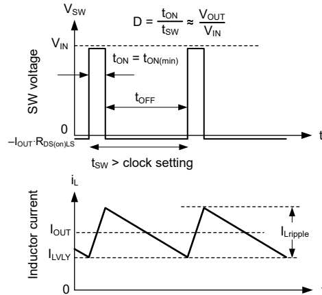
图 8-24. Valley Current Operation
