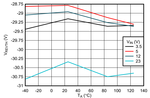
图 7-18. RCB - Reverse Comparator Threshold vs Temperature
