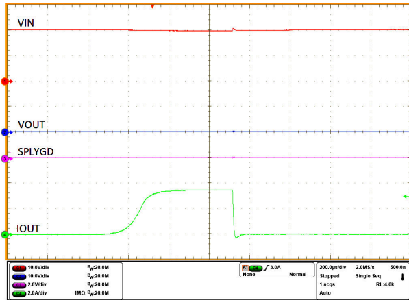
图 9-9. Wake up into Short Protection
