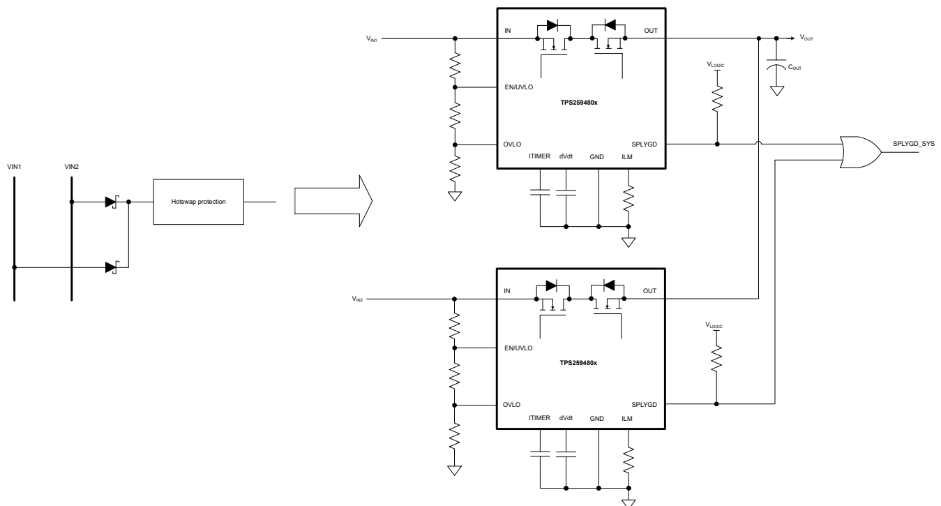
图 9-11. Two Devices, Active ORing Configuration
