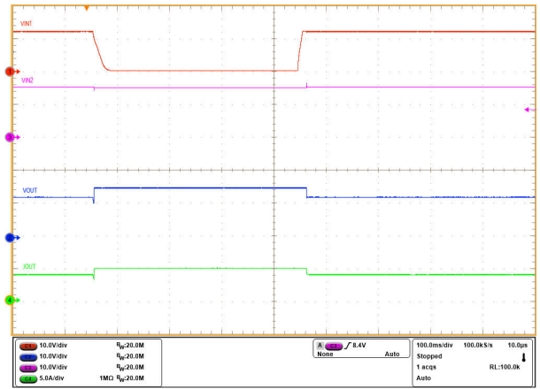
图 9-16. TPS25948x Power MUX - Switchover Between Primary and Auxiliary Supplies
