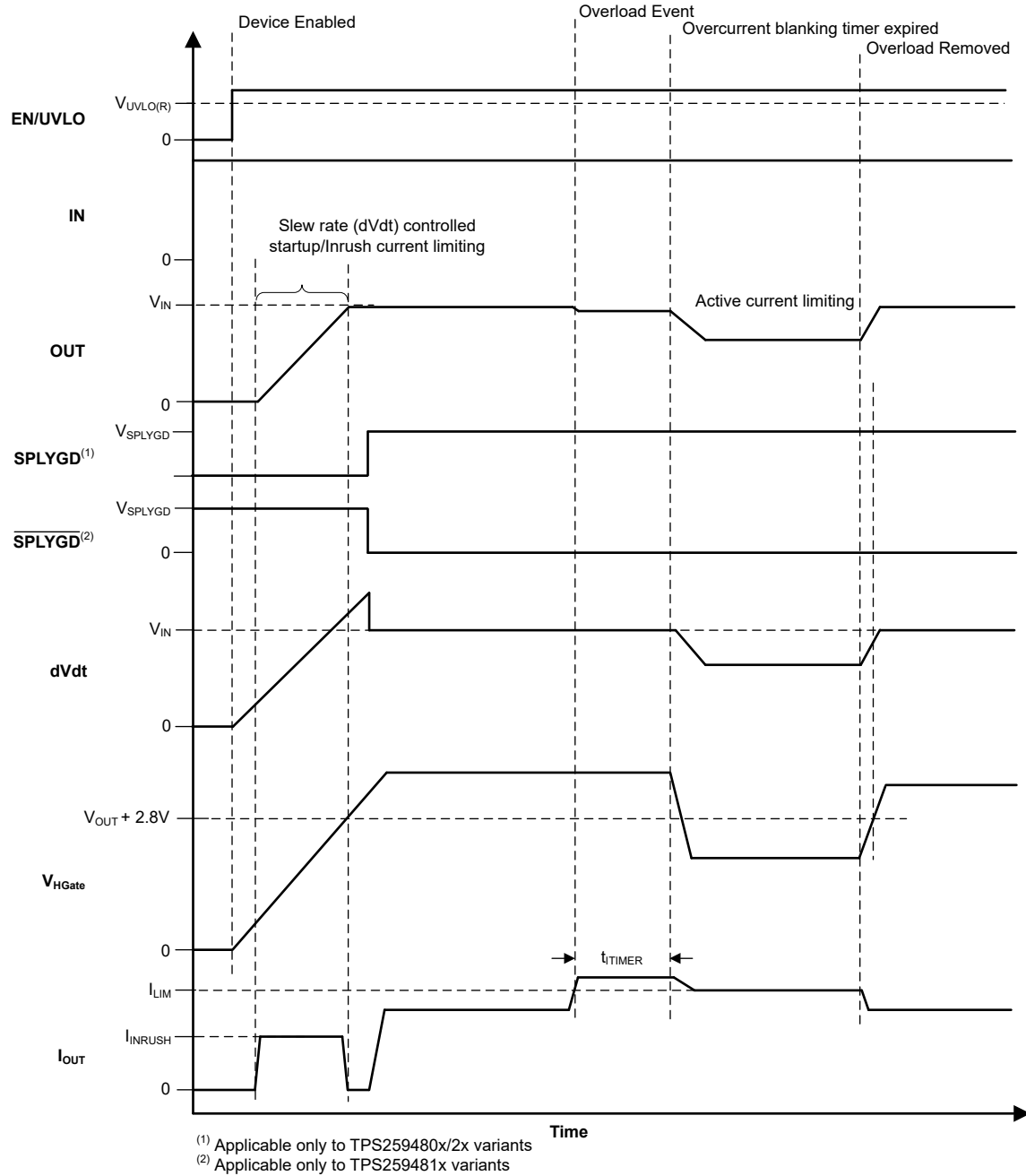
图 8-15. TPS25948xx SPLYGD Behavior
