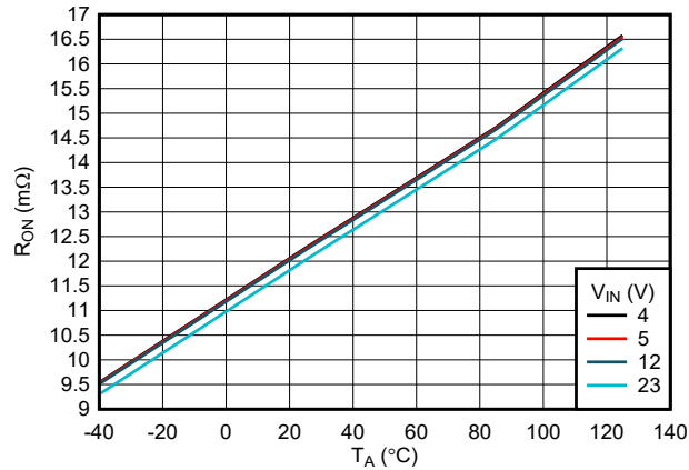
图 7-1. ON-Resistance vs Temperature
