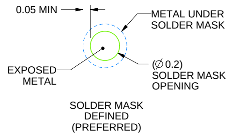
SOLDER MASK DETAILS NOT TO SCALE
