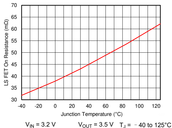
图 8-4. Low side R_{ds(on)} vs Junction Temperature
