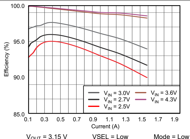
图 10-3. TPS61281D Efficiency vs Output Current
