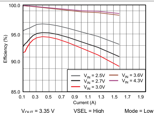
图 10-5. TPS61281D Efficiency vs Output Current
