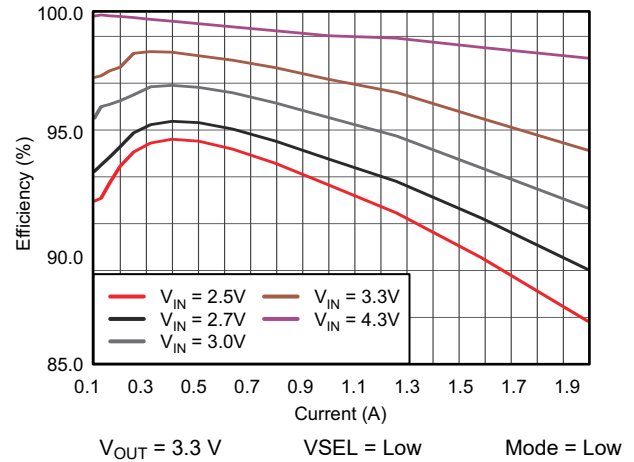
图 10-23. TPS61282D Efficiency vs Output Current
