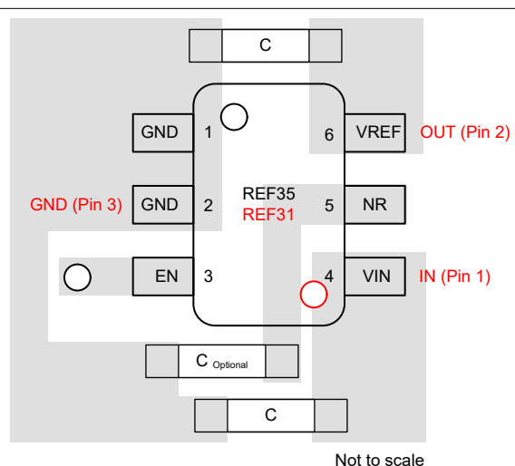
图 10-4. Pin Compatibility With REF31xx
