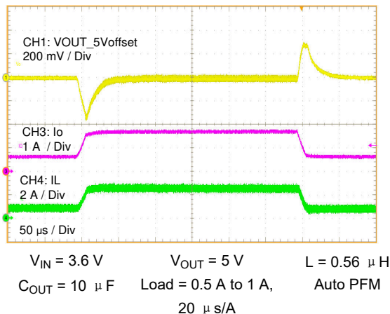
图 9-8. Load Transient with 10 \mu F C_{OUT}
