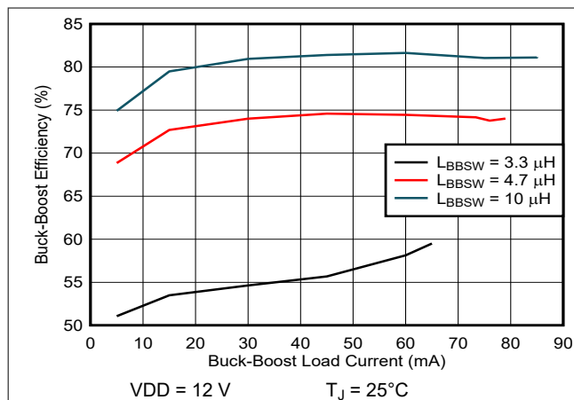
图 8-3. Buck-Boost Efficiency vs Load When I_{BBSW,PK} = I_{BBSW,PK(low)}
