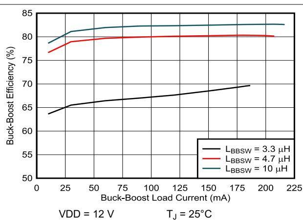
图 8-4. Buck-Boost Efficiency vs Load When I_{BBSW,PK} = I_{BBSW,PK(high)}
