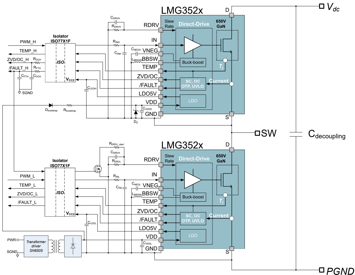
图 8-2. Typical Half-Bridge Application With Bootstrap
