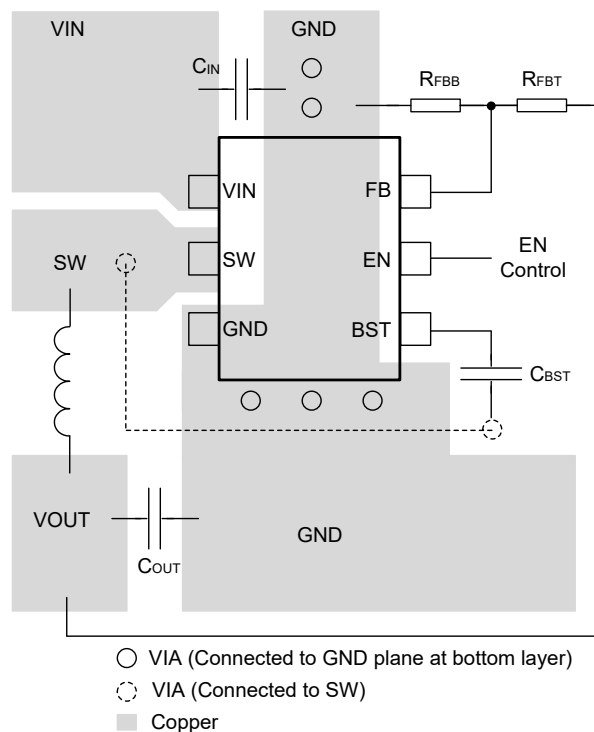
图 8-16. Suggested Layout
