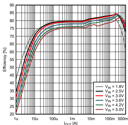
图 8-2. Efficiency at V_{OUT} = 0.4V
