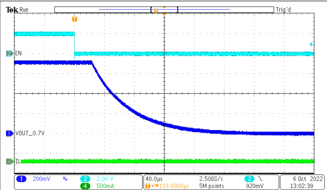
图 8-27. Shutdown, Output Discharge at V_{OUT} = 0.7V
