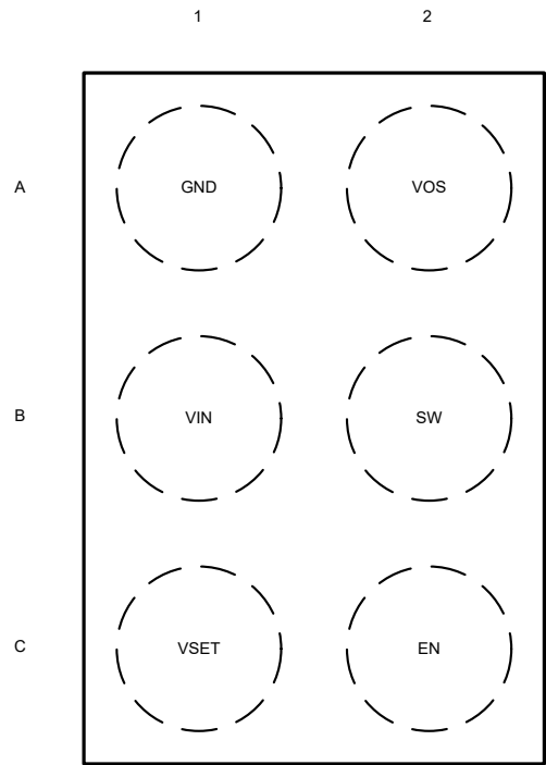
图 5-1. 6-Pin DSBGA YKA Package (Top View)
