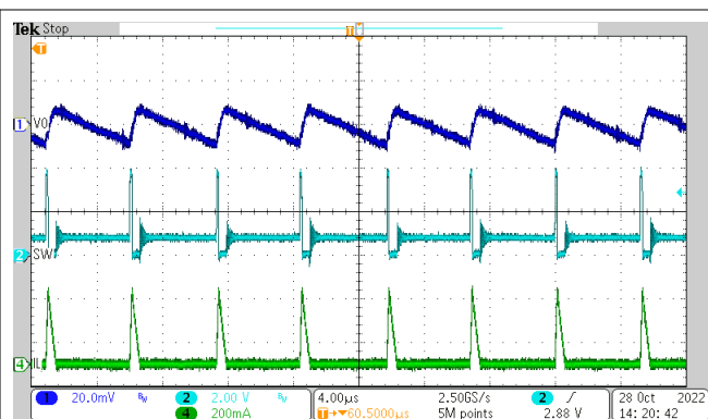
图 8-15. Typical Operation at V_{OUT} = 0.7V , I_{OUT} = 20mA
