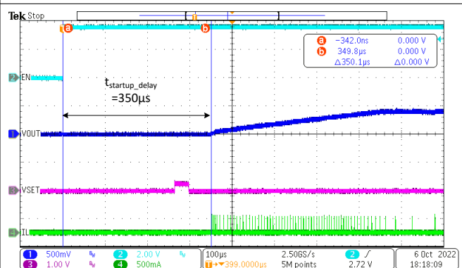
图 8-29. Start-Up Delay Time, V_{SET} = 10kohms
