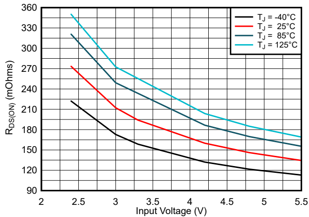
图 6-3. High Side Switch Drain Source Resistance R_{DS(ON)}
