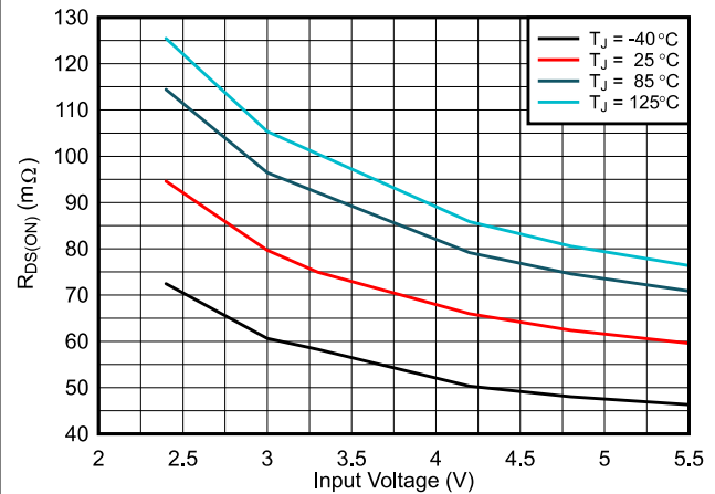
图 6-4. Low Side Switch Drain Source Resistance R_{DS(ON)}
