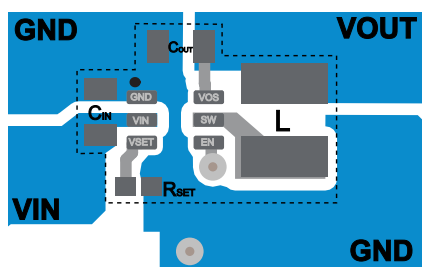
图 8-31. Layout Example (DRL Package)
