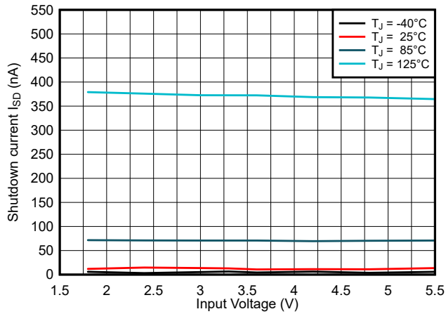
图 6-1. Shutdown Current I_{SD}
