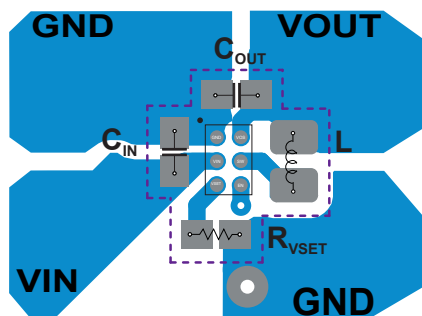
图 8-30. Layout Example (YKA Package)
