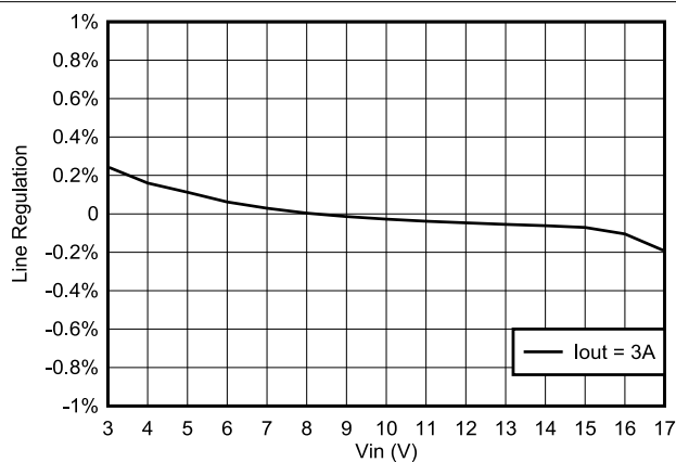
图 8-6. TPS563252 Line Regulation vs V_{IN}
