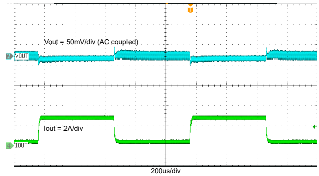
图 8-11. TPS563252 Transient Response with 0.3 A to 2.7 A
