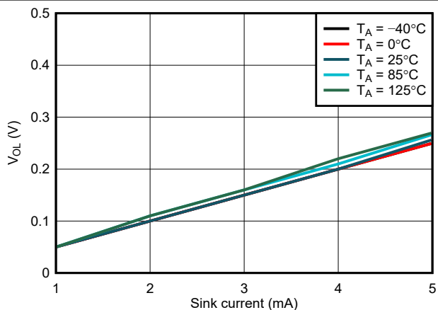
图 7-13. WDO V_{OL} vs I_{sink} , V_{DD} = 3.3\text{ V}
