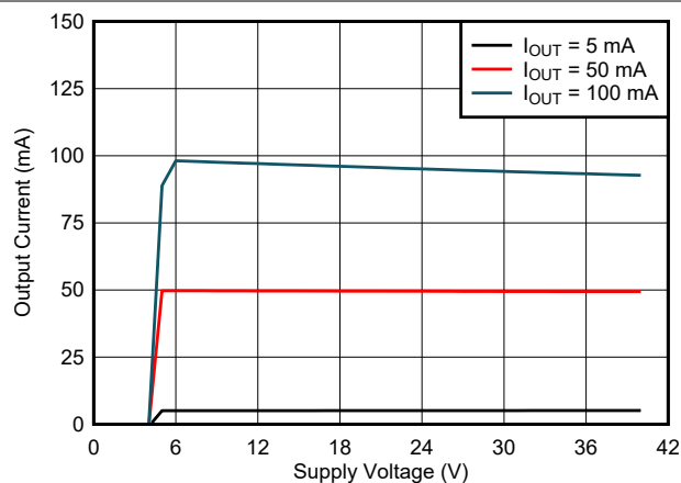
图 5-5. Output Current vs Supply Voltage
