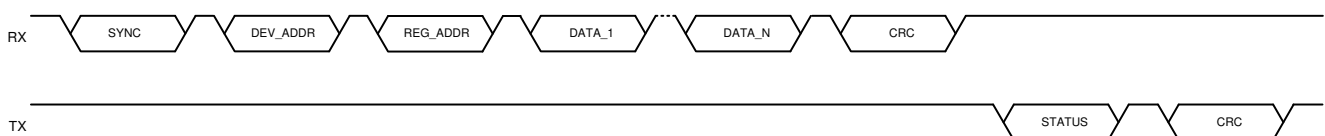
图 6-16. Multiple Data Bytes Write in Burst Mode
