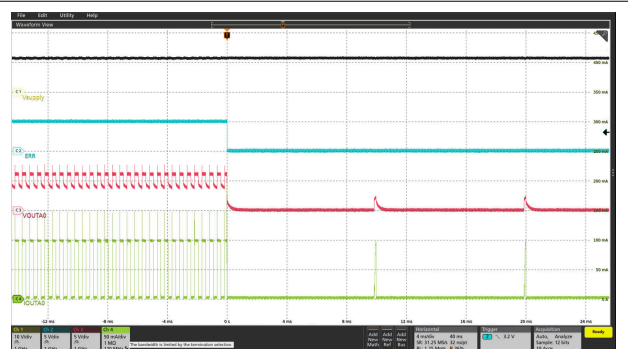
图 5-30. LED Short-Circuit Detection in Fail-Safe Mode
