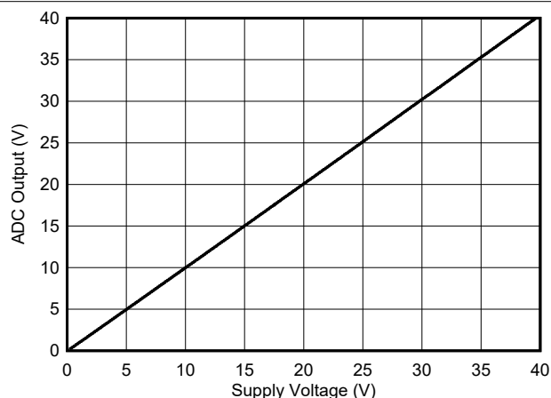
图 5-10. ADC Sampling Result vs Sampled Supply Voltage
