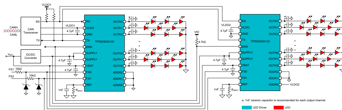
图 7-2. Typical Application Schematic
