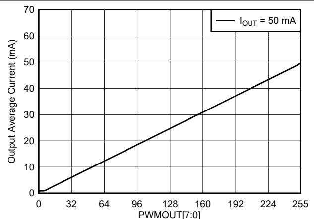
图 5-6. Average Current vs PWMOUT[7:0]
