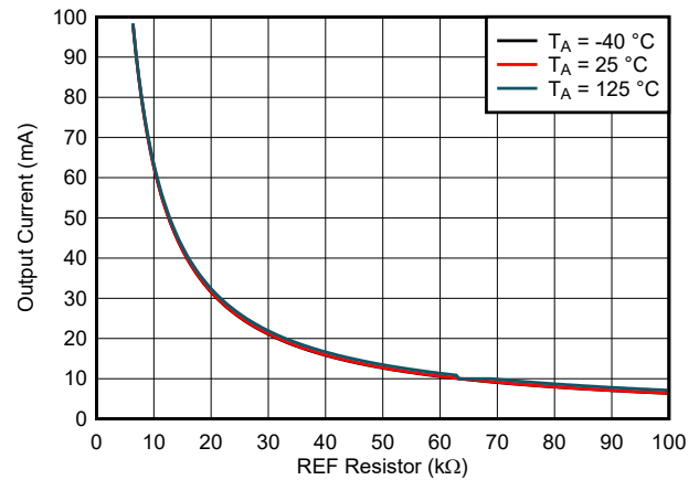
图 5-2. Output Current vs REF Resistor
