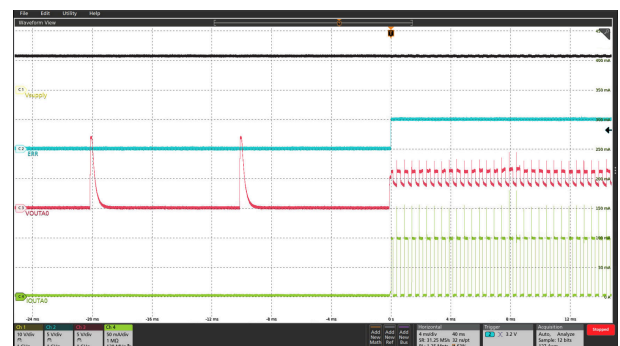
图 5-27. Single-LED Short-Circuit Detection in Normal Mode
