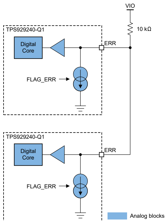
图 6-8. ERR Internal Block Diagram
