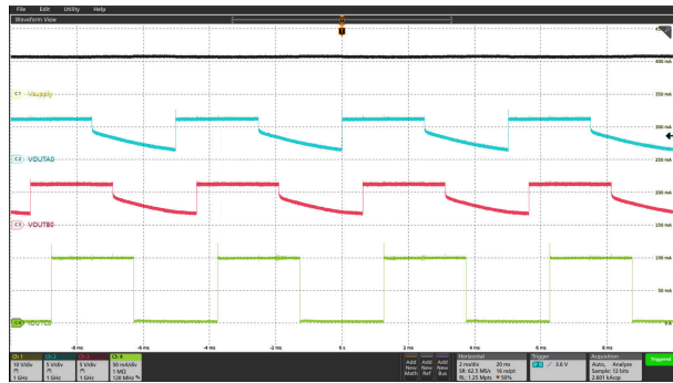
图 5-12. PWM Dimming at 200Hz
