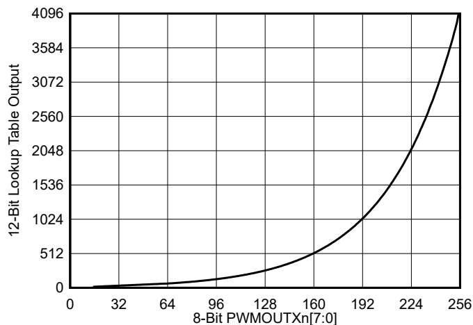
图 6-5. PWM Duty Cycle vs 8-Bit Code for Exponential Dimming
