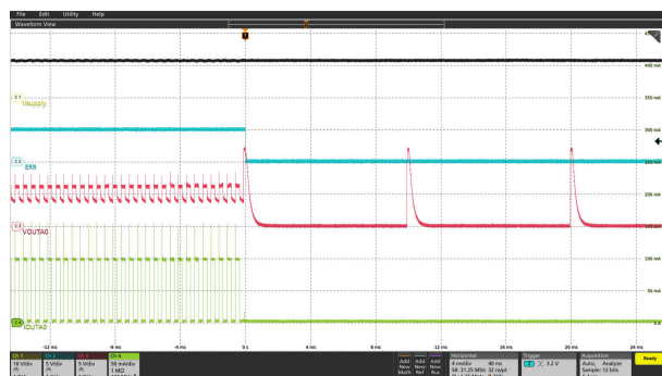
图 5-26. LED Short-Circuit Detection in Normal Mode
