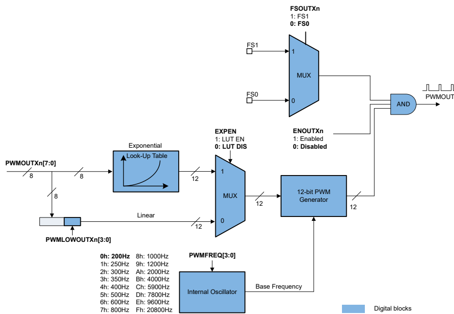
图 6-6. Output Current Control Path in FAIL-SAFE State
