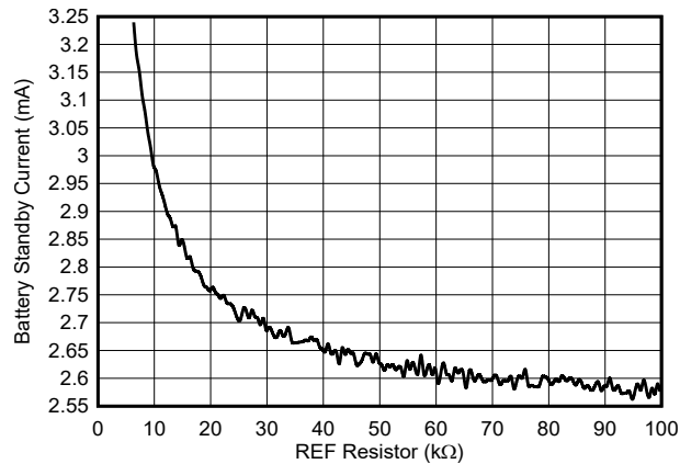
图 5-1. Standby Current vs REF Resistor
