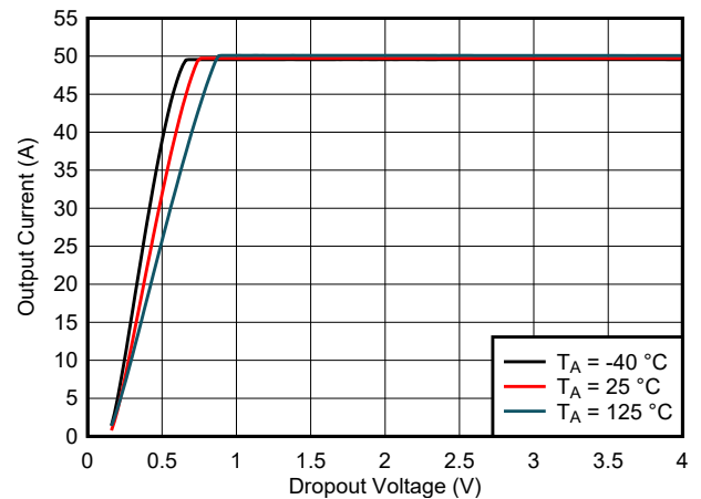
图 5-4. Output Current vs Dropout Voltage
