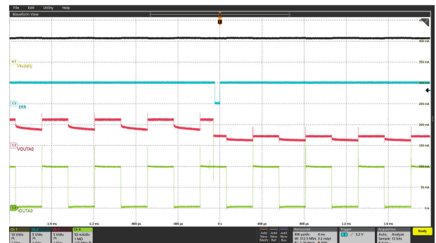
图 5-25. LED Open-Circuit Detection in Normal Mode
