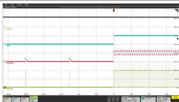
图 5-31. LED Short-Circuit Recovery in Fail-Safe Mode
