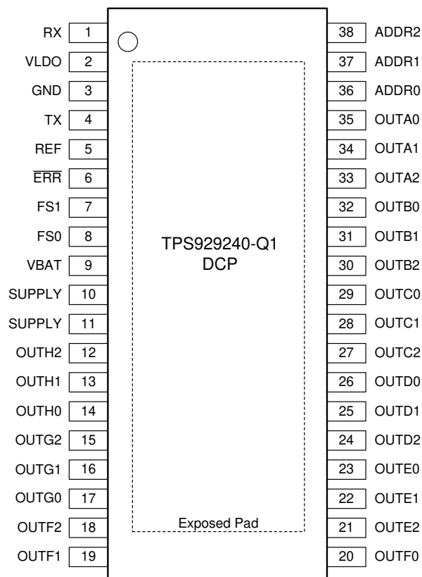
图 4-1. DCP Package 38-Pin HTSSOP with PowerPAD™ Integrated Circuit Package Top View
