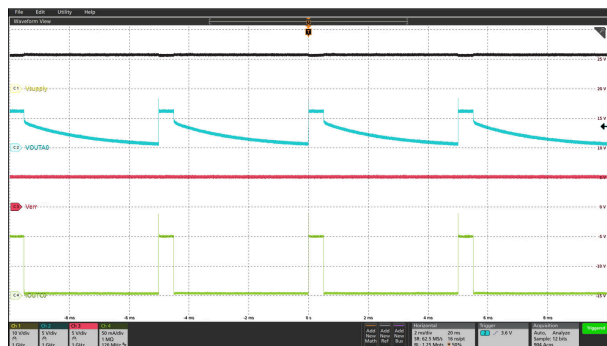
图 5-14. Phase Shift PWM Dimming at 200Hz
