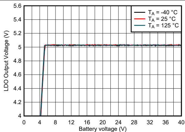
图 5-8. LDO Output Line Regulation
