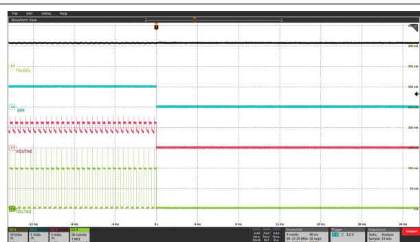
图 5-30. LED Short-Circuit Detection in Fail-Safe Mode
