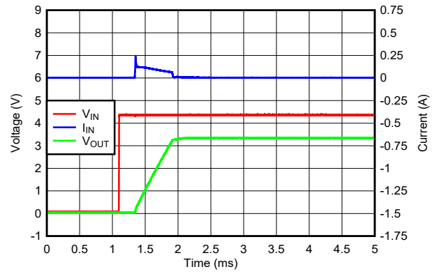
图 5-20. Inrush Current With 22\text{ }\mu\text{F} at C_{OUT}
