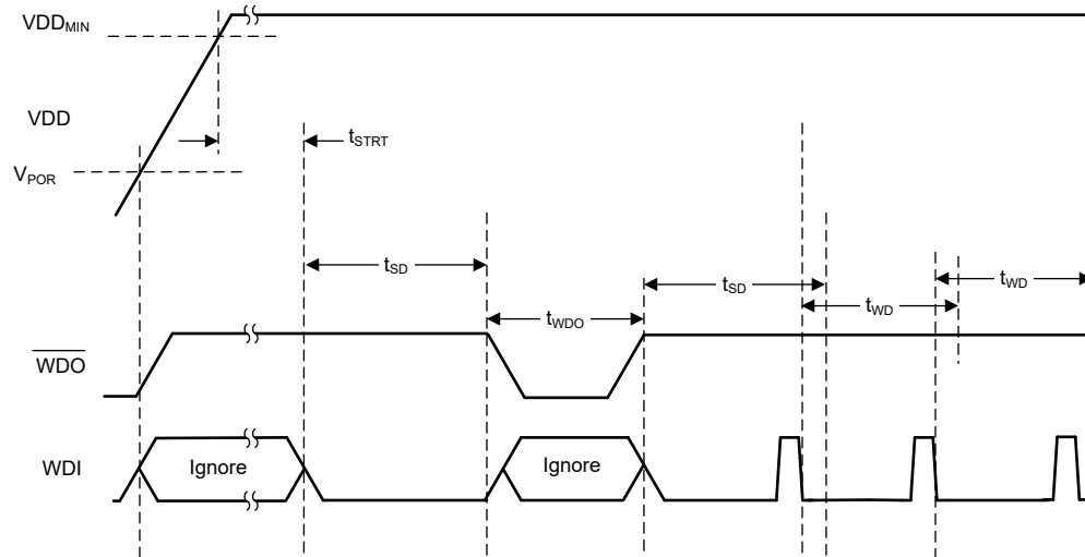
图 8-8. t_{SD} Frame Behavior
