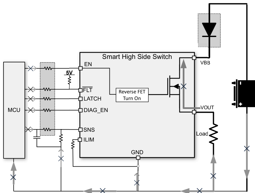
图 8-22. Reverse Protection with Blocking Diode
