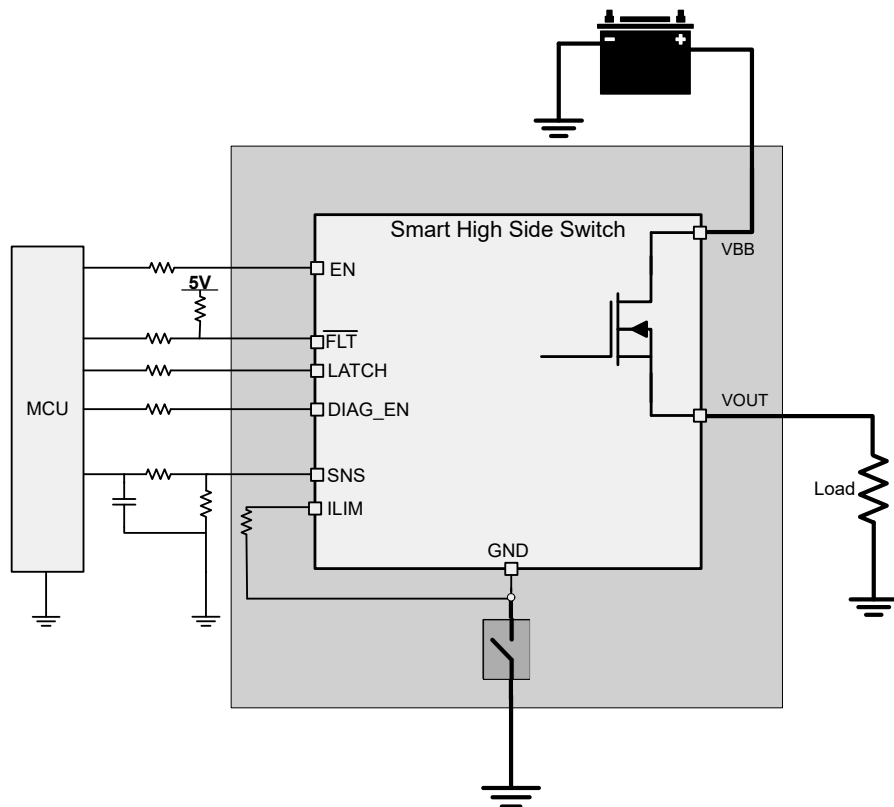
图 8-19. Loss of Device GND
