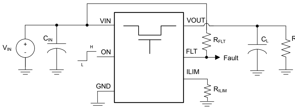
图 9-1. Typical Application
