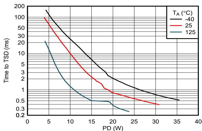
图 8-2. Time to Thermal Shutdown vs Power Dissipation
