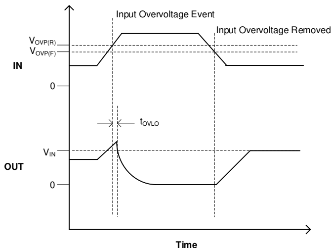
图 7-2. TPS25961 Fixed Overvoltage Lockout Response
