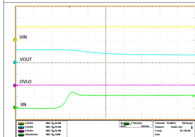
图 8-12. Overcurrent Protection
