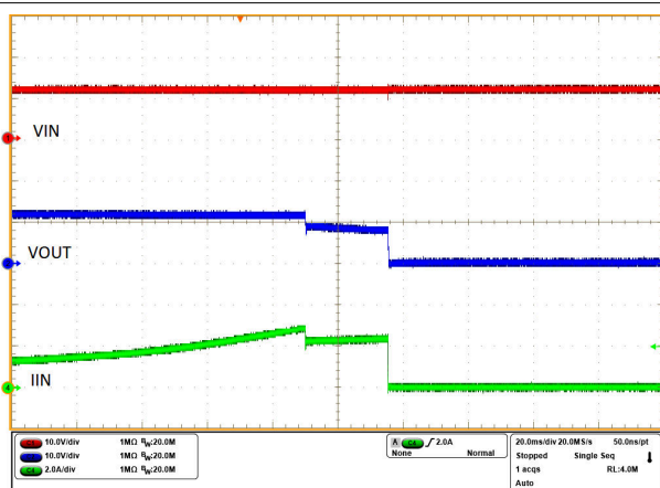
图 8-5. Overcurrent Protection
