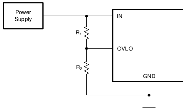
图 7-4. TPS25961 Adjustable Overvoltage Lockout
