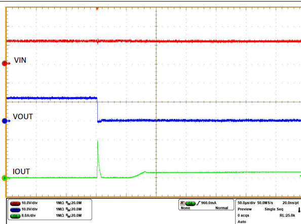
图 8-6. Short at Output Protection
