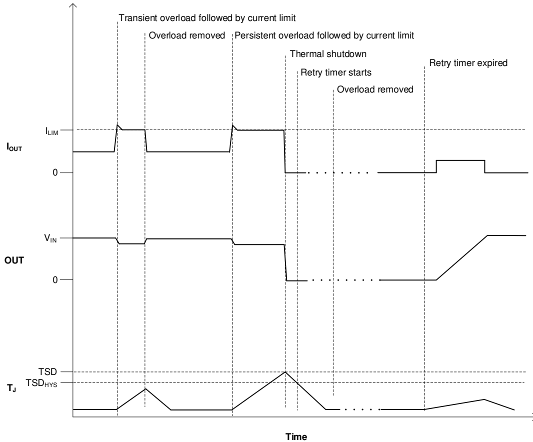
图 7-5. TPS25961 Overcurrent Response
