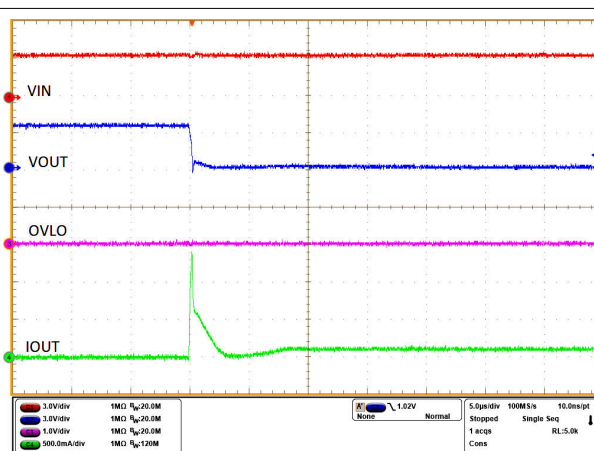
图 8-13. Short at Output Protection
