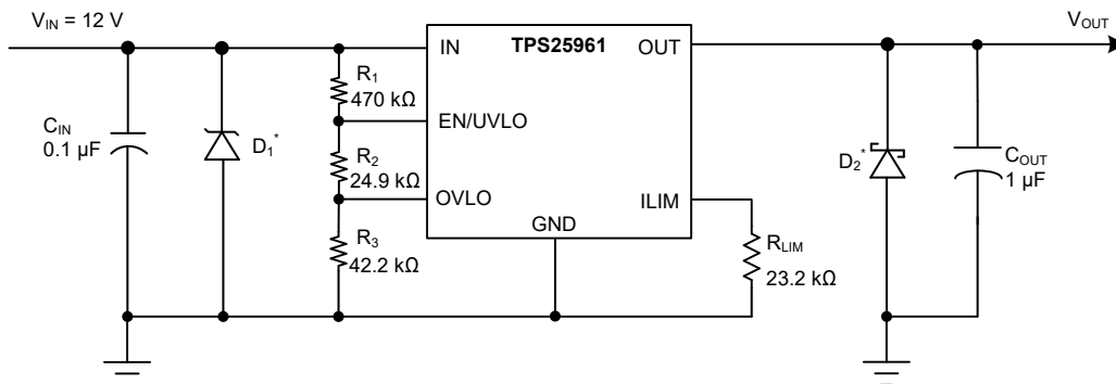
图 8-1. Typical Application Schematic
