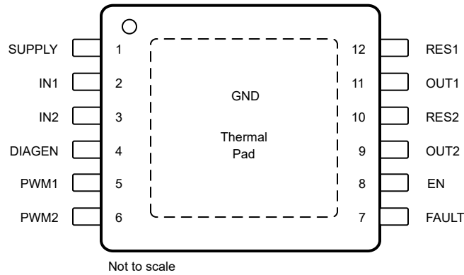
图 4-1. DGN Package 12-Pin HVSSOP With PowerPAD™ Integrated Circuit Package (Top View)
