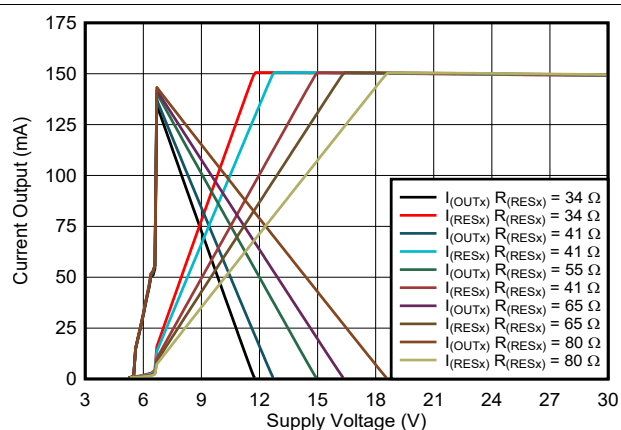
图 5-6. Output Current Distribution vs Supply Voltage
