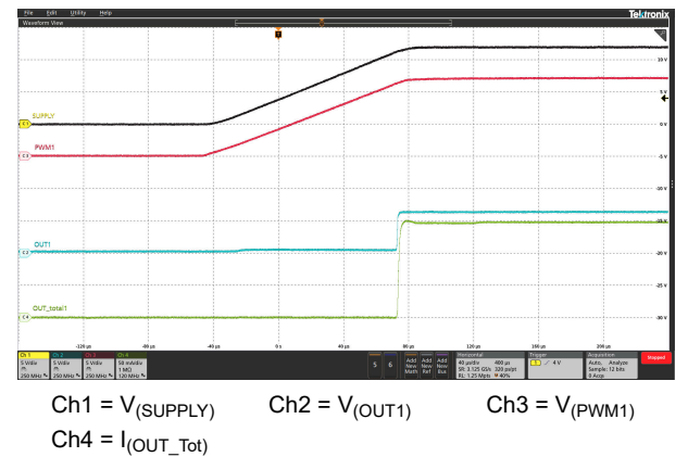
图 5-10. Power-Up Sequence
