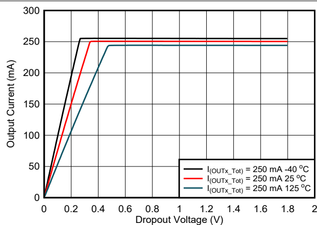
图 5-3. Output Current vs Dropout Voltage
