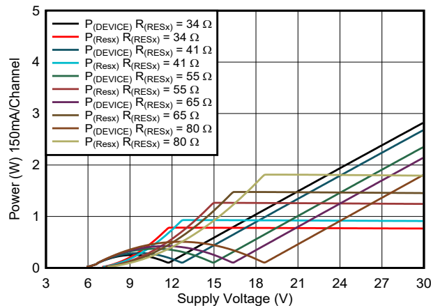
图 5-7. Power Dissipation vs Supply Voltage
