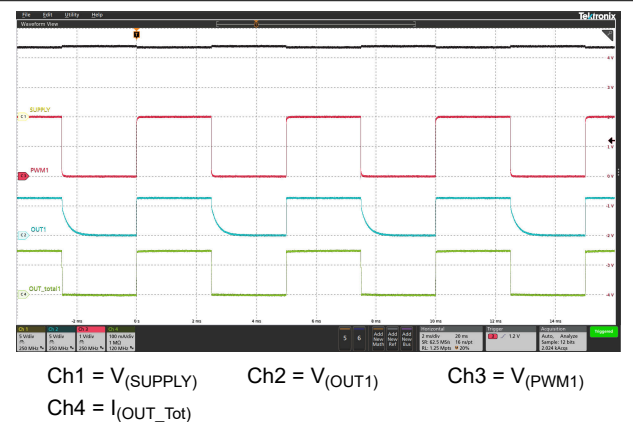
图 5-12. PWM Dimming at 200 Hz
