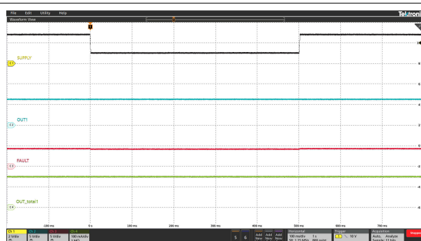
图 5-16. LED Short-Circuit Protection
