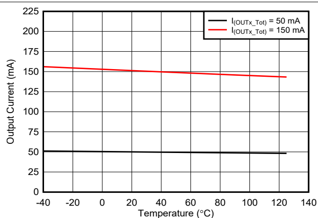
图 5-2. Output Current vs Temperature
