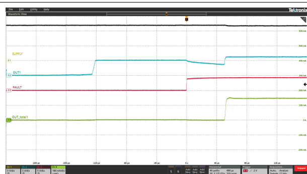
图 5-15. LED Open Protection Recovery
