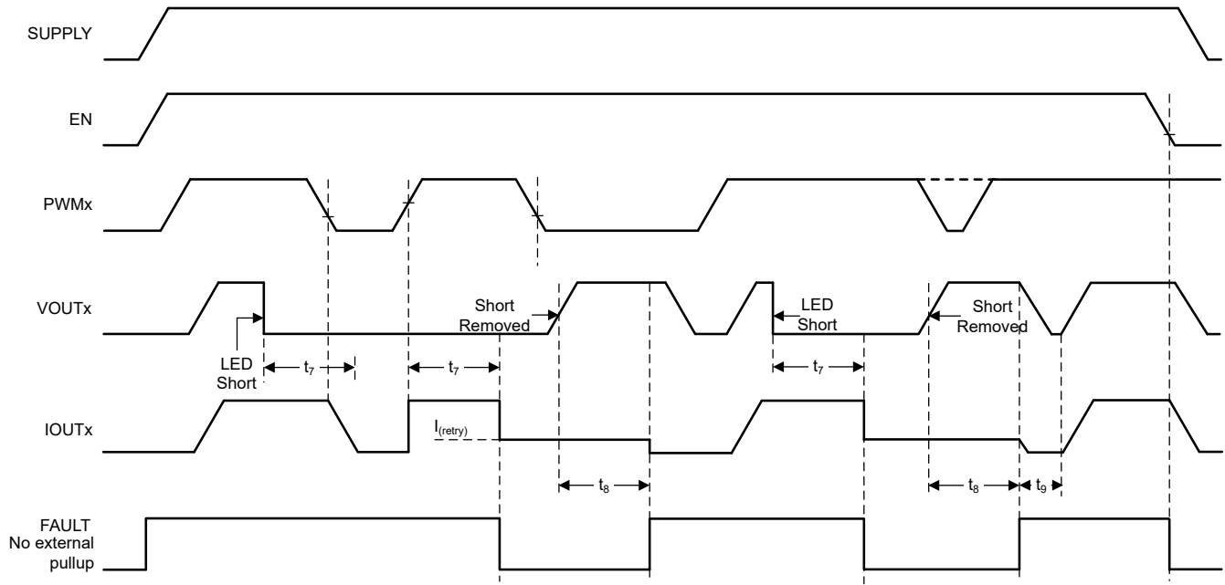
图 6-3. LED Short-to-GND Detection and Recovery Timing Diagram
