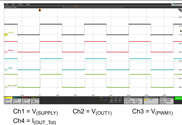
图 5-11. Supply Dimming at 200 Hz
