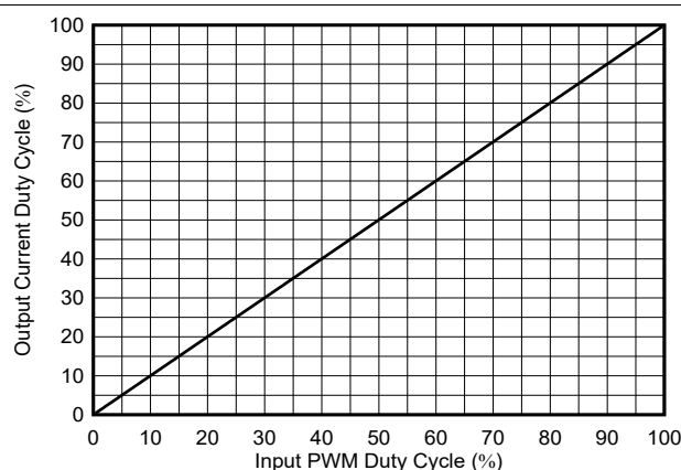
图 5-5. PWM Output Duty Cycle vs PWM Input Duty Cycle
