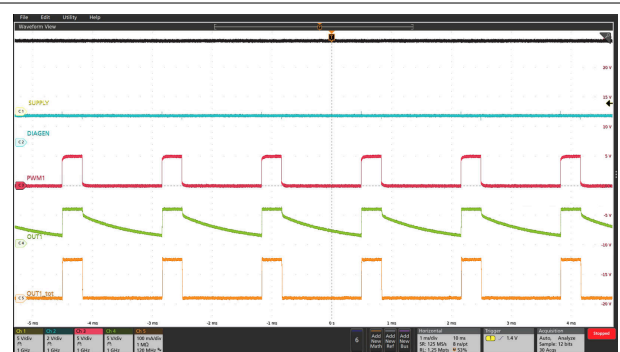
图 7-6. 600-Hz PWM Dimming at 20% Duty Cycle
