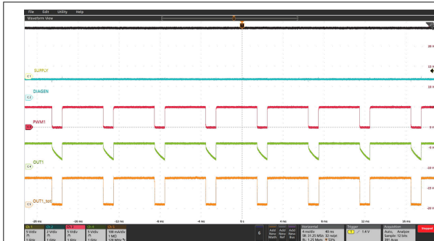
图 7-5. 200-Hz PWM Dimming at 80% Duty Cycle
