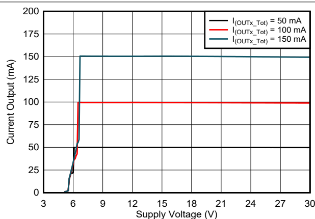
图 5-1. Output Current vs Supply Voltage
