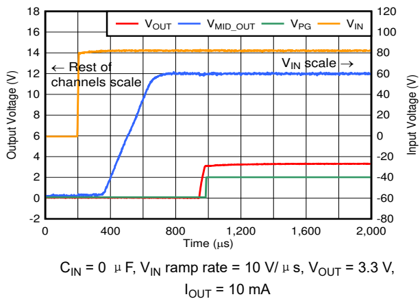
图 6-12. Fast Start-Up
