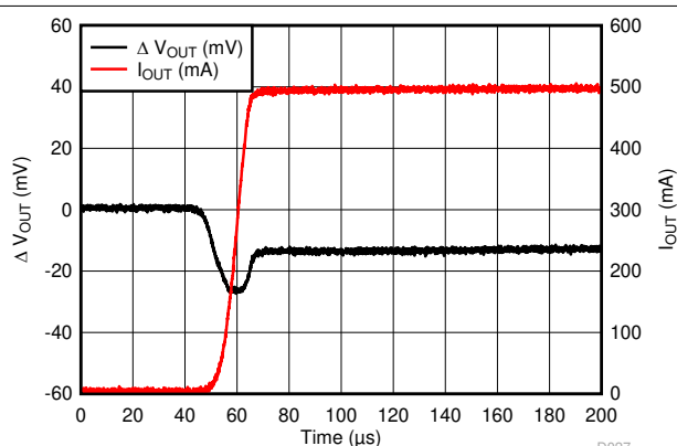
图 6-34. LP5912-1.8 Load Transient Response
