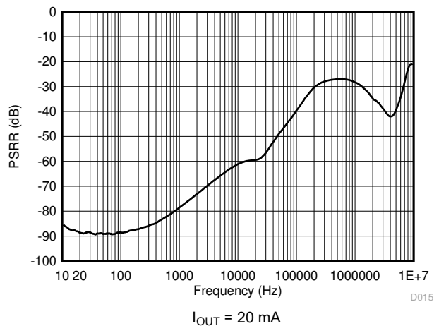
图 6-24. LP5912-3.3 PSRR vs Frequency
