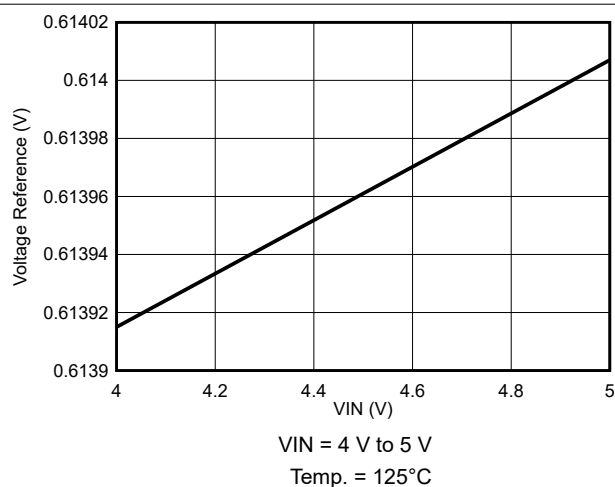
图 7-15. Voltage Reference Variation
