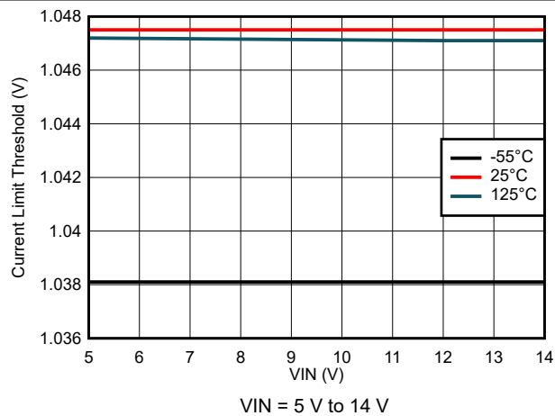
图 7-18. Current Limit Threshold Variation
