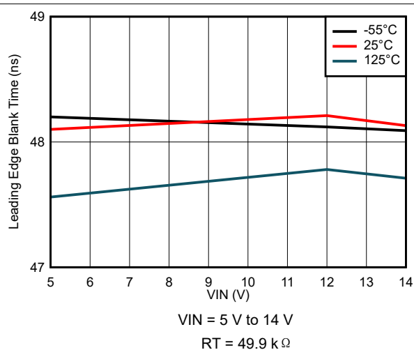
图 7-36. Leading Edge Blank Time Variation
