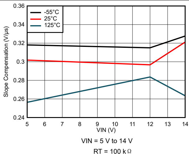
图 7-70. Slope Compensation Variation
