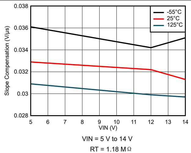
图 7-66. Slope Compensation Variation
