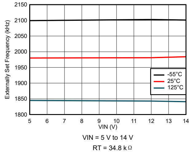
图 7-26. Externally Set Frequency Variation
