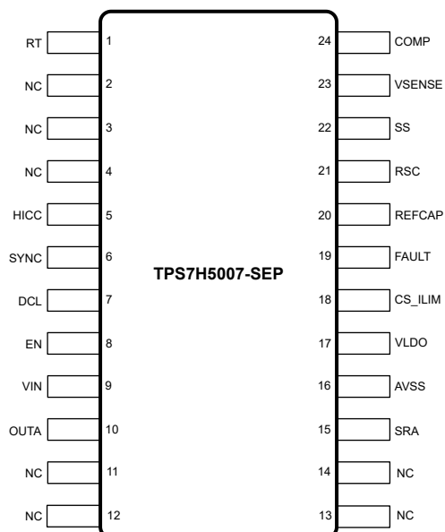
图 6-3. TPS7H5007-SEP PW Package 24-Pin TSSOP (Top View)
