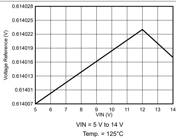
图 7-16. Voltage Reference Variation
