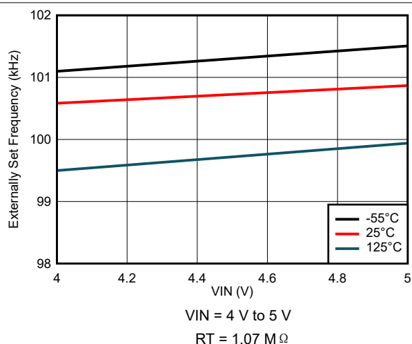
图 7-19. Externally Set Frequency Variation
