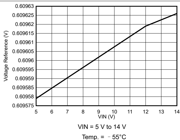
图 7-12. Voltage Reference Variation
