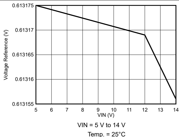
图 7-14. Voltage Reference Variation
