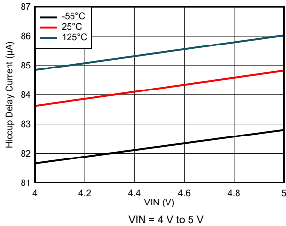
图 7-27. Hiccup Delay Current Variation
