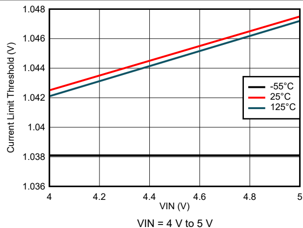
图 7-17. Current Limit Threshold Variation
