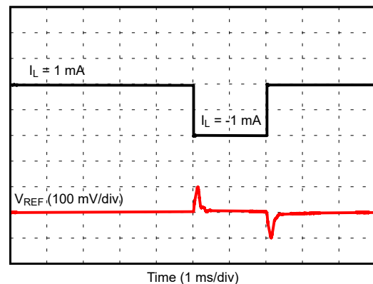
图 6-24. Load Transient Response ( V_{REF} = 2.5\text{V} , C_L = 1\mu\text{F} )
