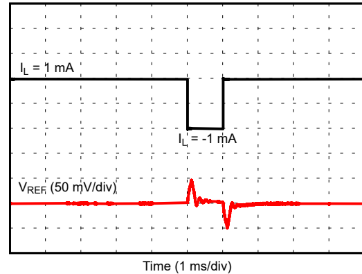
图 6-22. Load Transient Response ( V_{REF} = 2.5\text{V} , C_L = 10\mu\text{F} )
