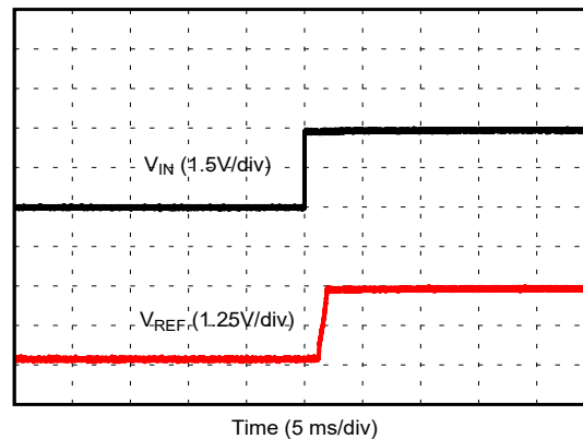
图 8-2. REF35250 Start-Up Behavior, C_L = 1 \mu F
