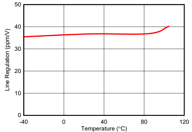
图 6-28. Line Regulation vs Free-Air Temperature
