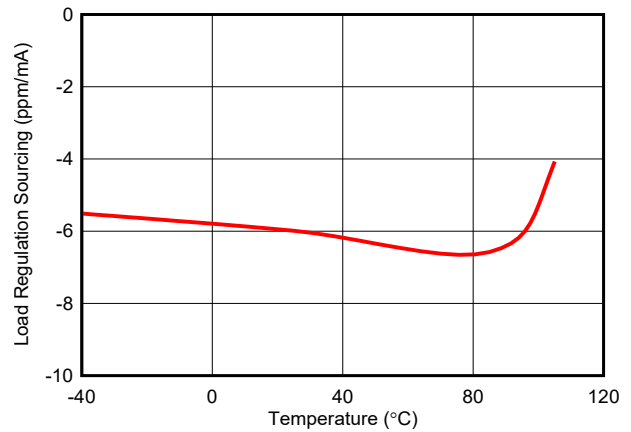
图 6-20. Load Regulation (Sourcing 10mA) vs Free-Air Temperature
