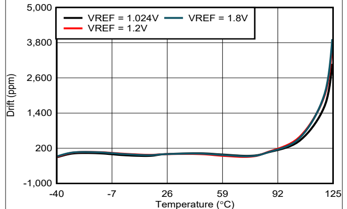
图 6-6. Output Voltage Drift vs Free-Air Temperature
