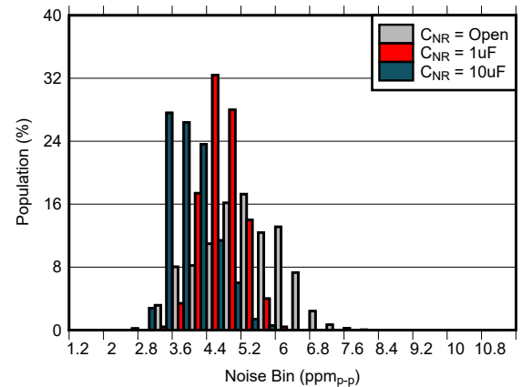
图 7-14. 0.1Hz to 10Hz Noise Distribution vs NR Capacitance
