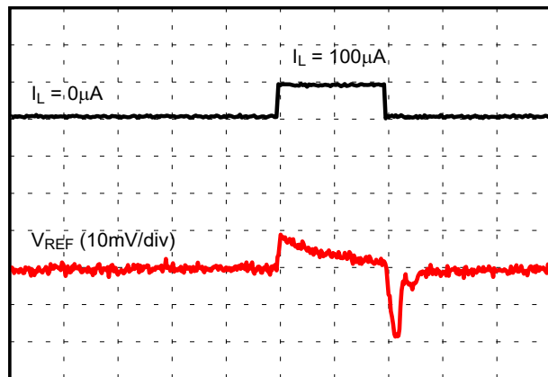
图 8-3. Load Transient Response 0 \mu A to 100 \mu A , C_L = 1 \mu F
