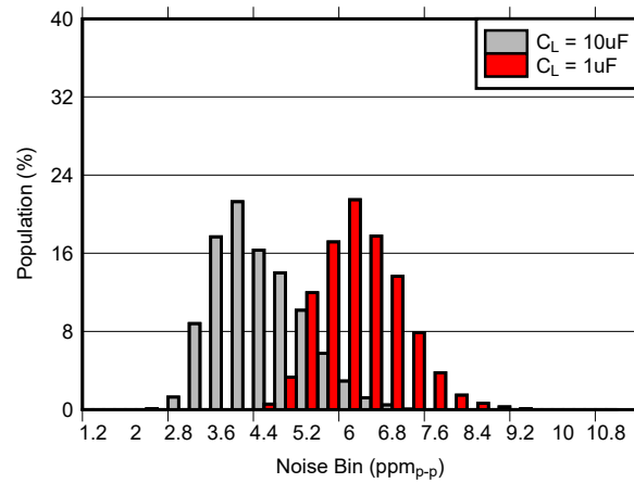
图 6-14. 0.1Hz to 10Hz Noise Distribution ( V_{REF} = 5\text{V} , C_{NR} = \text{Open} , I_L = 0\text{mA} )
