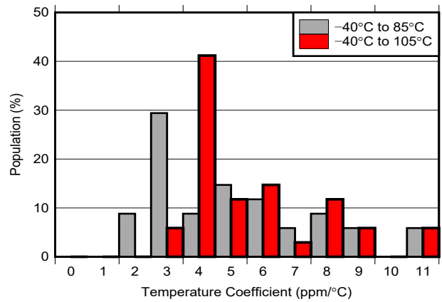
图 6-4. Temperature Coefficient Distribution ( V_{REF} = 5.0\text{V} )
