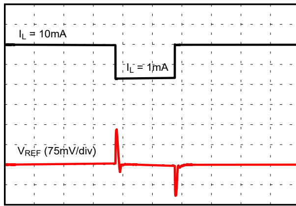
图 8-4. Load Transient Response 1 mA to 10 mA , C_L = 1 \mu F
