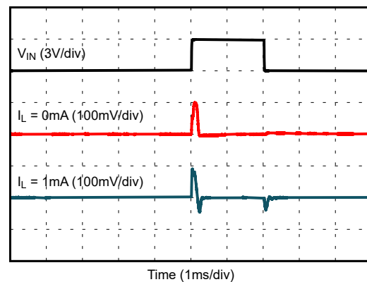
图 6-30. Line Transient Response ( V_{REF} = 2.5\text{V} , C_L = 1\mu\text{F} )
