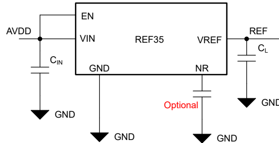
图 8-1. Basic Connections
