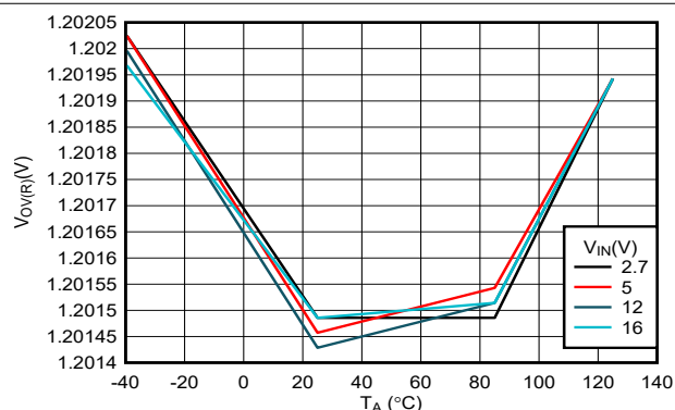
图 6-11. EN/OVLO Rising Threshold vs Temperature
