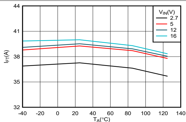
图 6-13. Fixed Fast-Trip Threshold vs Temperature
