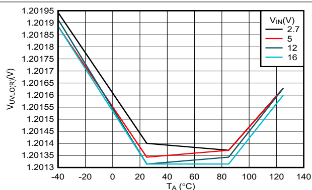
图 6-9. EN/UVLO Falling Threshold vs Temperature
