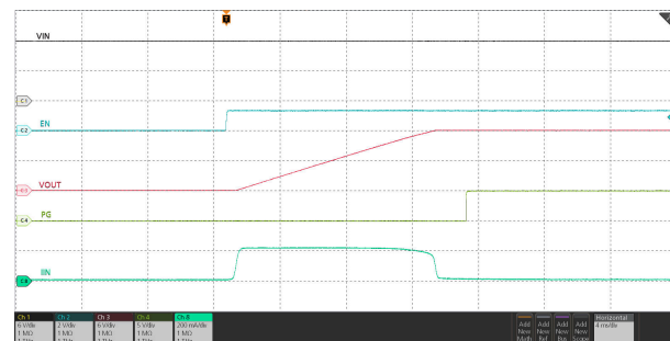
图 6-23. Start-Up with Enable
