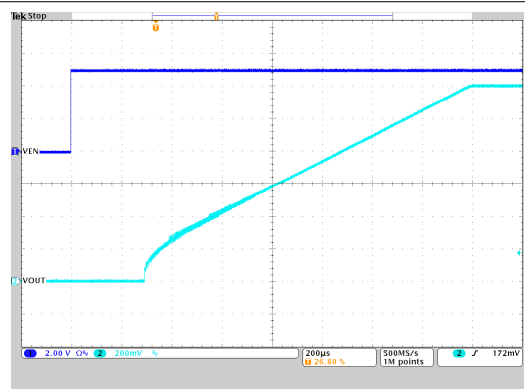
图 9-52. Start-Up Timing
