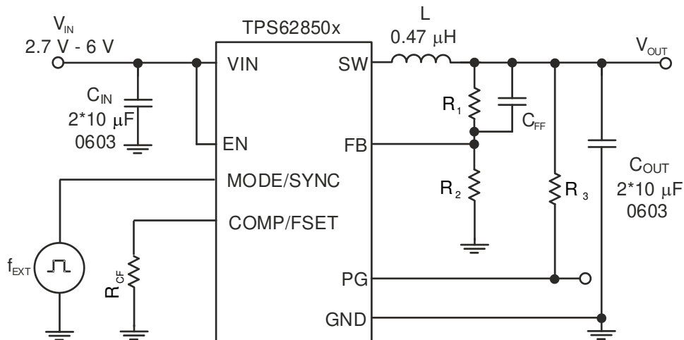
图 9-57. Schematic using External Synchronization
