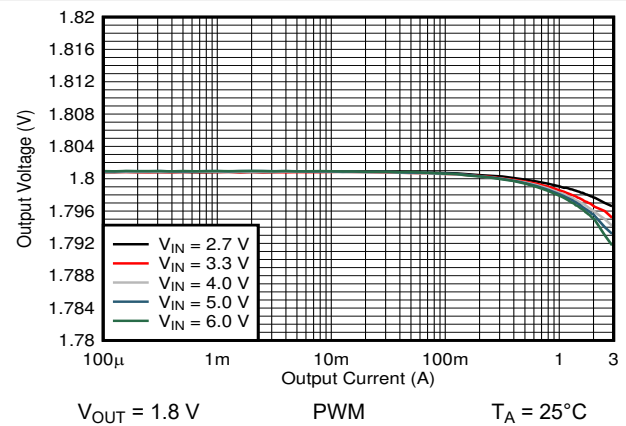
图 9-13. Output Voltage Versus Output Current
