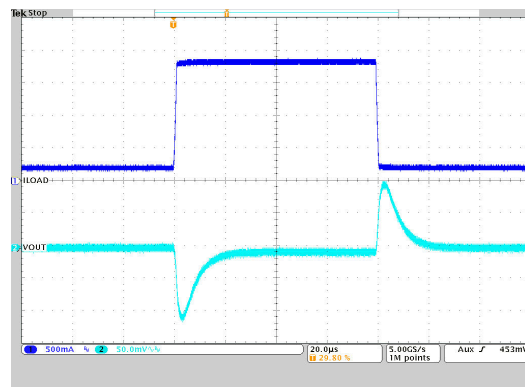
图 9-27. Load Transient Response
