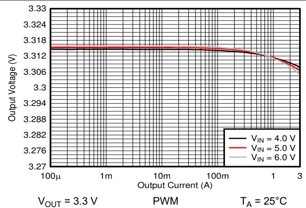
图 9-11. Output Voltage Versus Output Current
