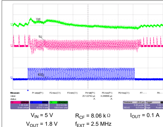
图 9-58. Switching from External Synchronization to Power-Save Mode (PFM)
