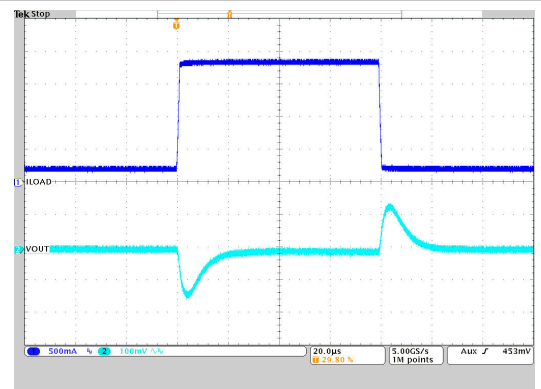
图 9-23. Load Transient Response
