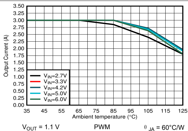
图 9-19. Output Current Versus Ambient Temperature
