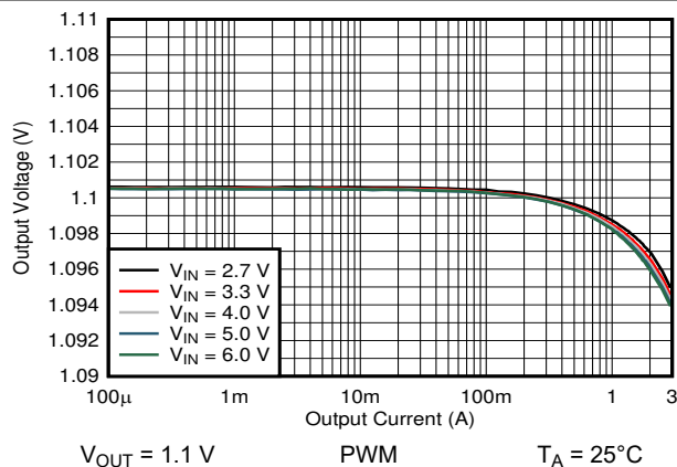
图 9-15. Output Voltage Versus Output Current
