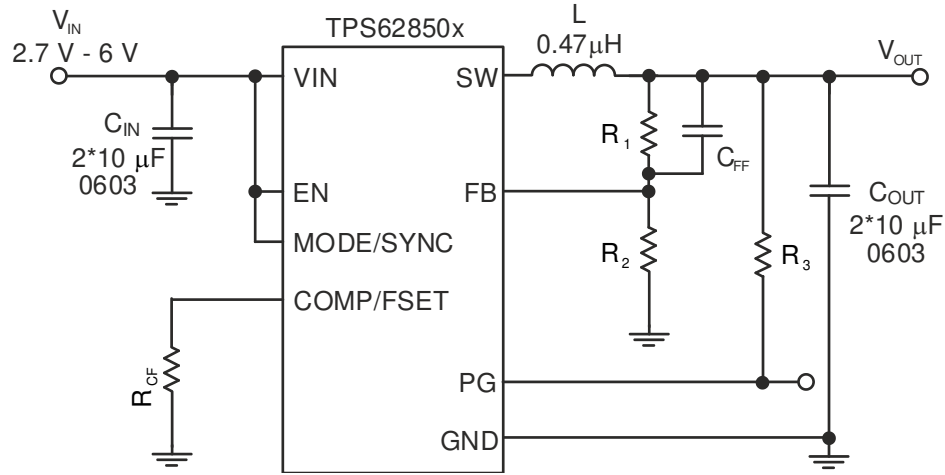
图 9-1. Typical Application
