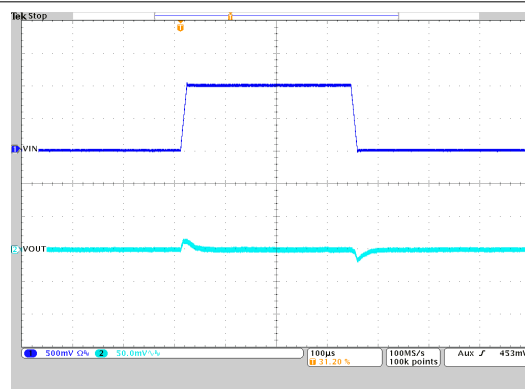
图 9-35. Line Transient Response
