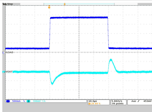
图 9-22. Load Transient Response
