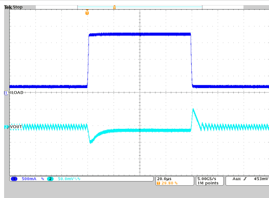
图 9-28. Load Transient Response
