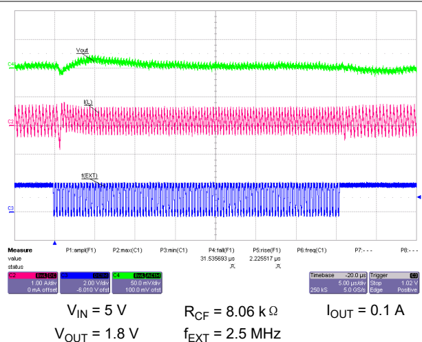
图 9-59. Switching from External Synchronization to Internal Fixed Frequency
