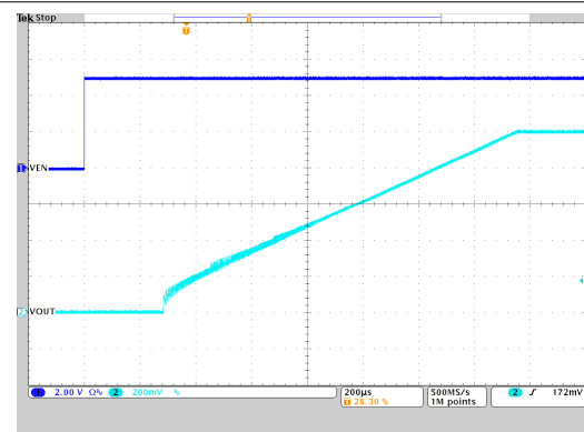
图 9-53. Start-Up Timing
