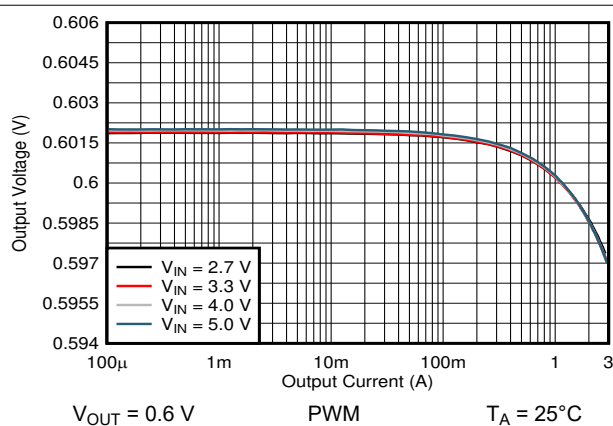
图 9-17. Output Voltage Versus Output Current
