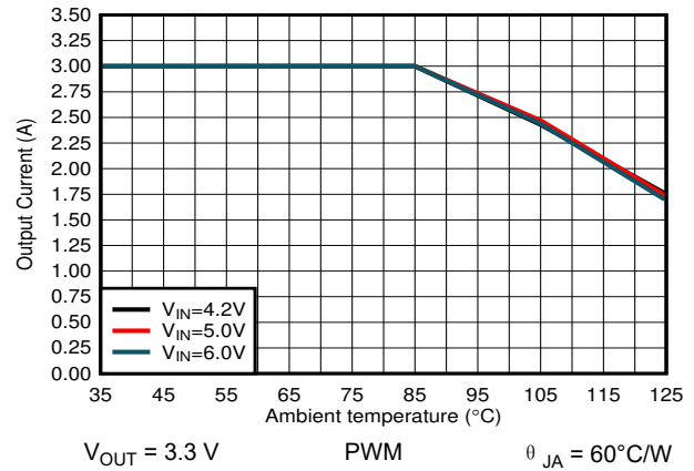
图 9-21. Output Current Versus Ambient Temperature
