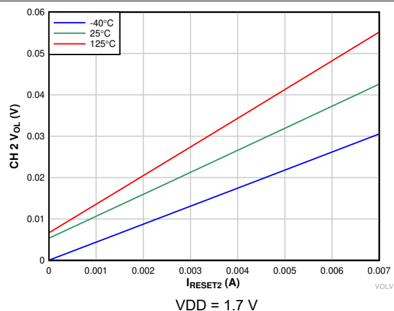
图 6-10. Low-Level CH 2 Output Voltage vs \overline{\text{RESET2}} Current
