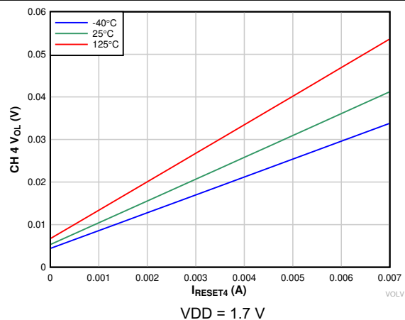
图 6-14. Low-Level CH 4 Output Voltage vs \overline{\text{RESET4}} Current
