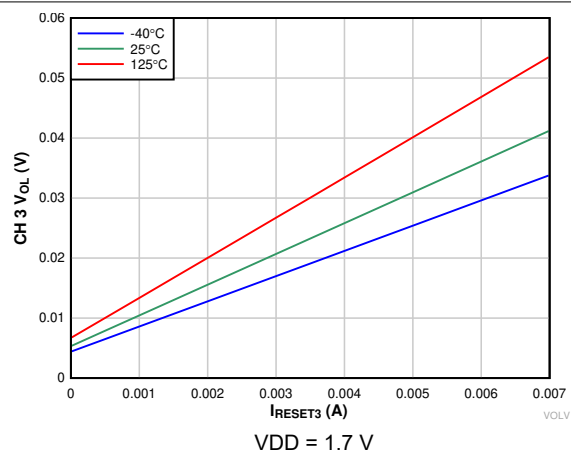
图 6-12. Low-Level CH 3 Output Voltage vs \overline{\text{RESET3}} Current
