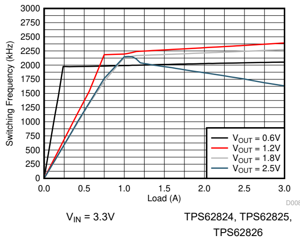
图 8-23. Switching Frequency
