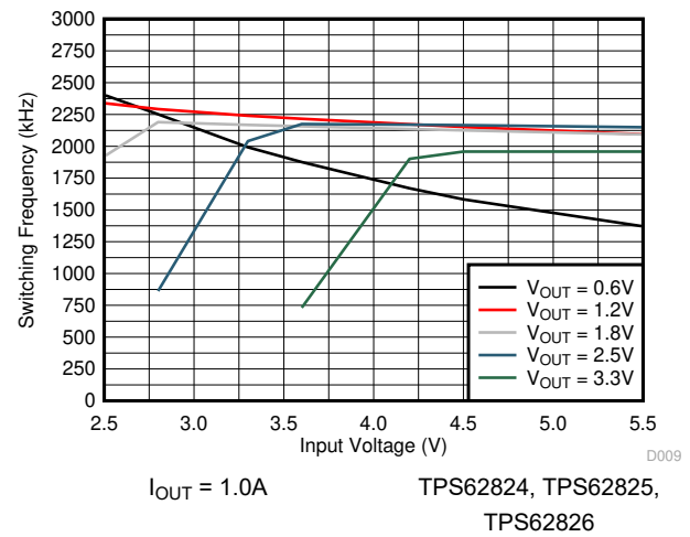
图 8-24. Switching Frequency
