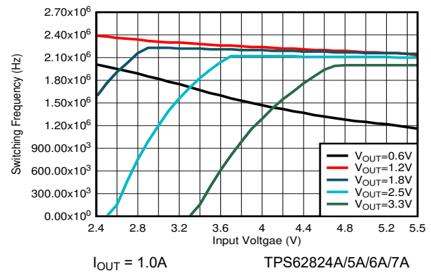
图 8-26. Switching Frequency
