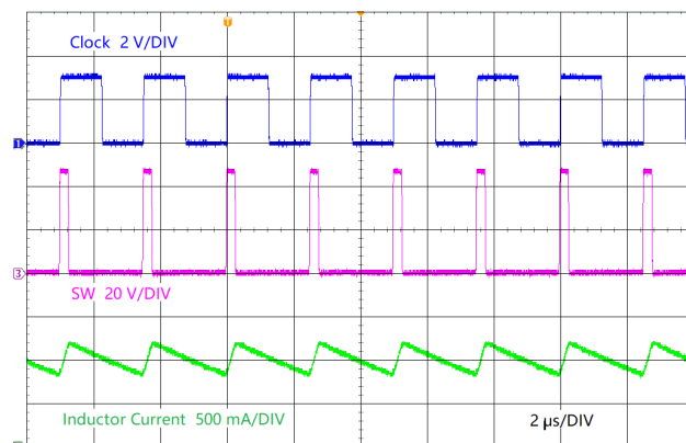
LMR38010 V_{OUT} = 5\text{ V} 400 kHz
