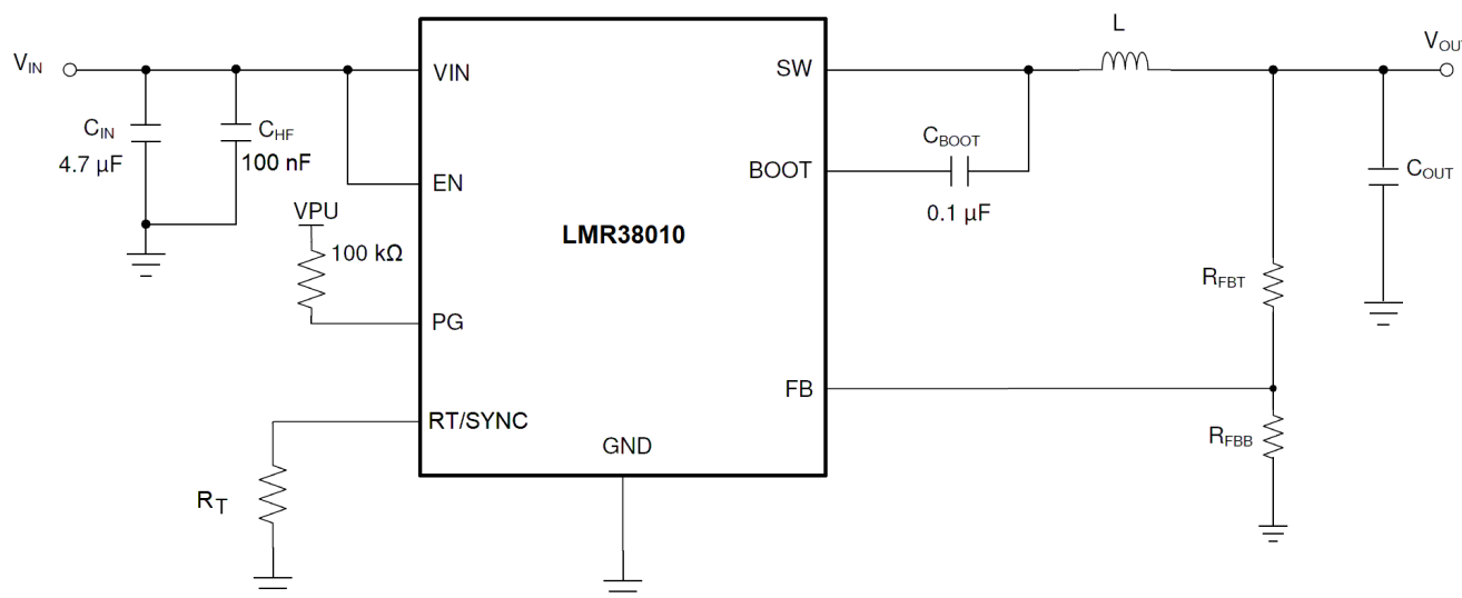
图 9-1. Example Application Circuit
