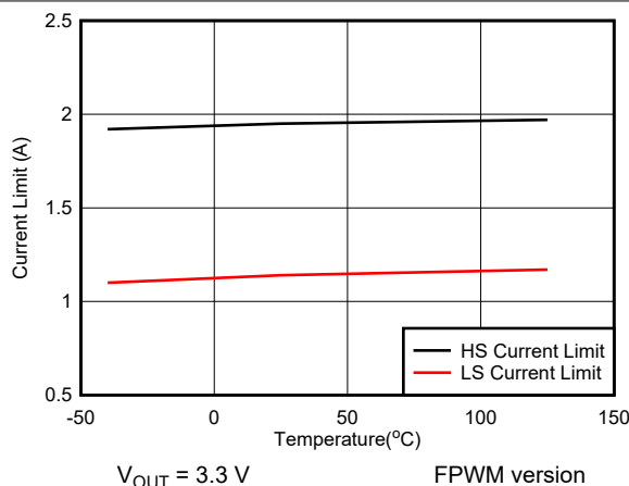
图 7-5. High-Side and Low-Side Current Limit vs Temperature
