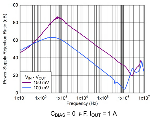
图 6-23. PSRR vs Frequency and V_{IN} - V_{OUT}
