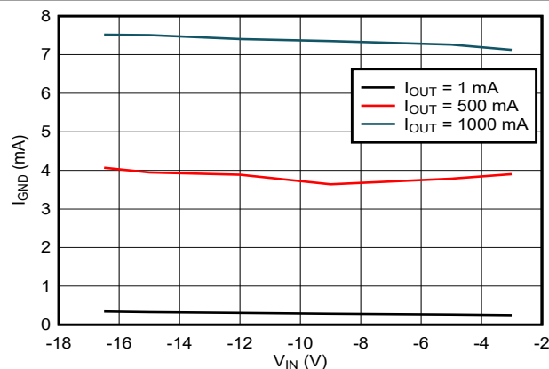
图 6-3. Ground Current vs Input Voltage Across Output Current
