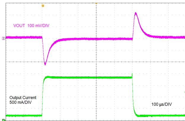
LMR38020 V_{OUT} = 5\text{ V} 400 kHz (AC Coupled)
