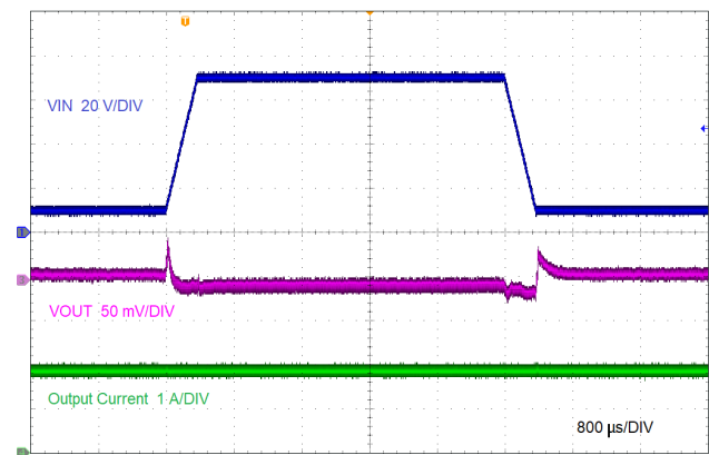
LMR38020 V_{OUT} = 5\text{ V} 400 kHz (AC Coupled)
