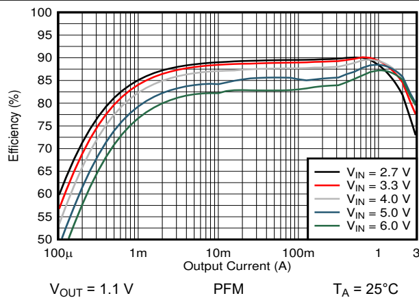
图 9-6. Efficiency Versus Output Current
