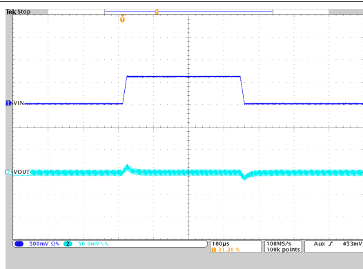
图 9-38. Line Transient Response
