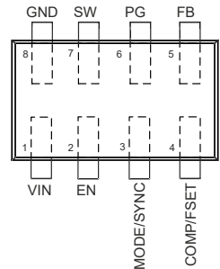
图 5-2. 8-Pin SOT583 DYC Package for TPS62850x-Q1 (Top View)
