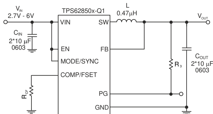
图 9-57. Schematic for Fixed Output Voltage Versions
