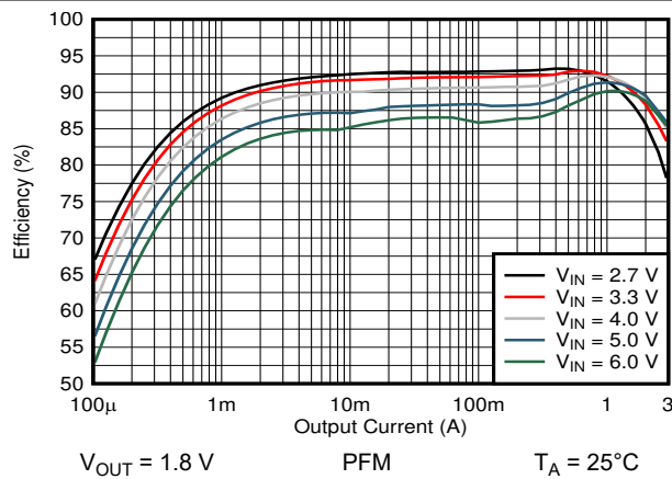
图 9-4. Efficiency Versus Output Current
