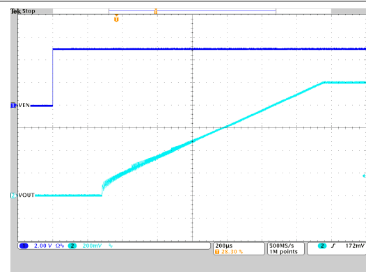
图 9-53. Start-Up Timing
