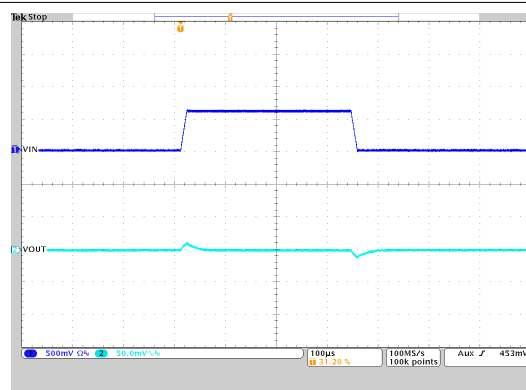
图 9-39. Line Transient Response
