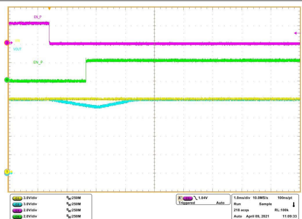
图 10-4. Switch From Primary to Secondary TPS7H2211 in a Cold Sparing Application
