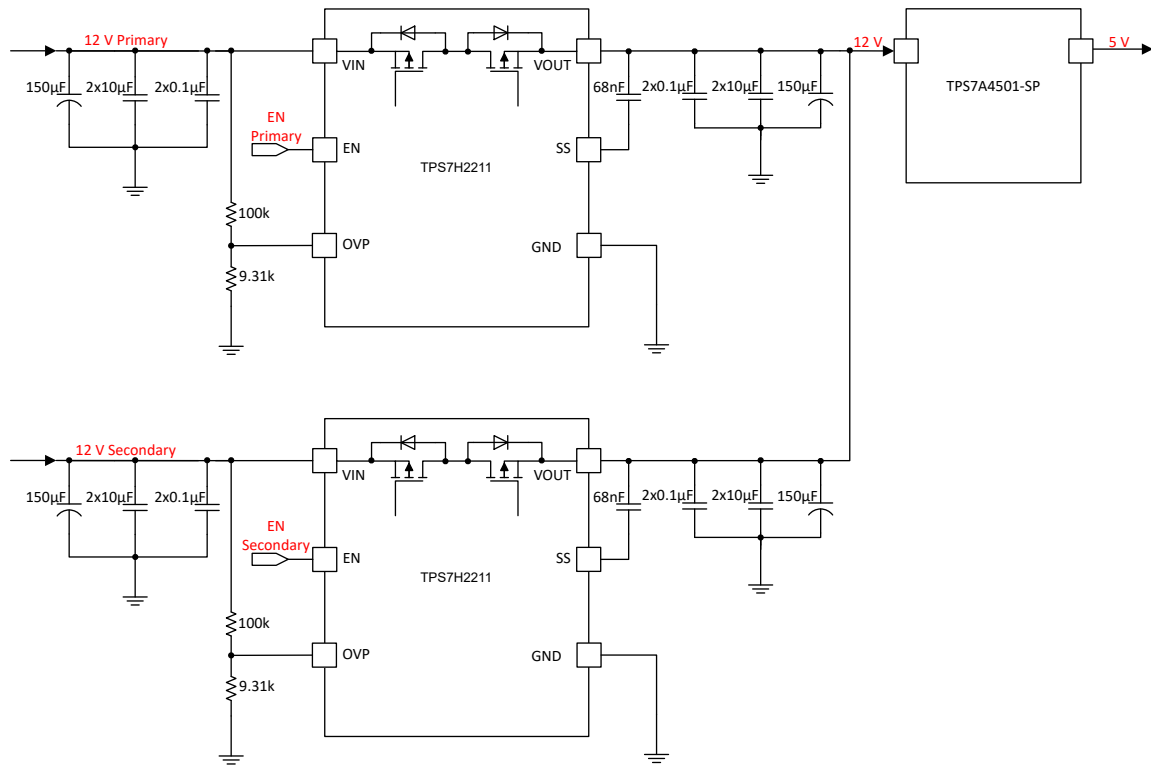
图 10-2. Cold Sparing Example With Calculated Component Values
