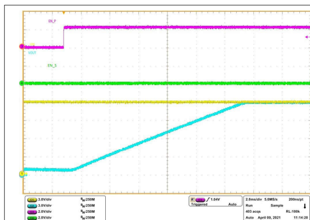
图 10-3. Power-Up Behavior of Primary TPS7H2211 in a Cold Sparing Application
