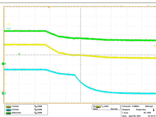
图 10-8. Undervoltage Turn-Off of TPS7H2211 in Protection Application
