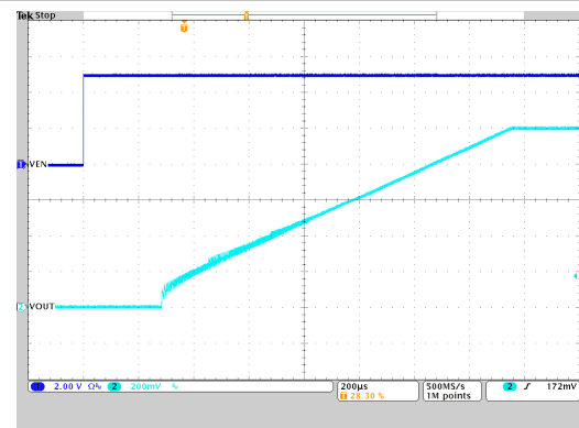
图 10-53. Start-Up Timing
