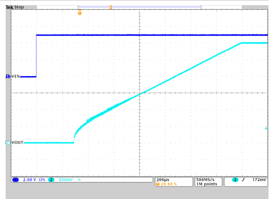
图 10-52. Start-Up Timing
