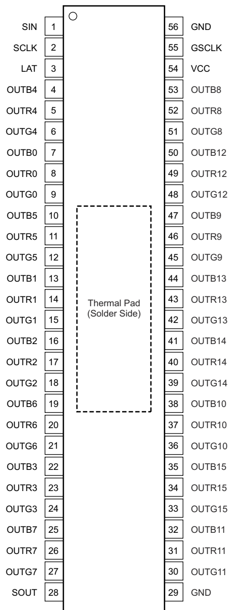
图 5-1. DCA Package HTSSOP-56 (Top View)
