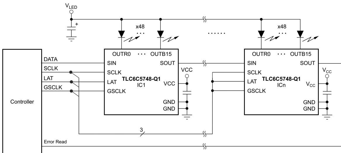
图 9-1. Multiple Daisy-Chained TLC6C5748-Q1 Devices
