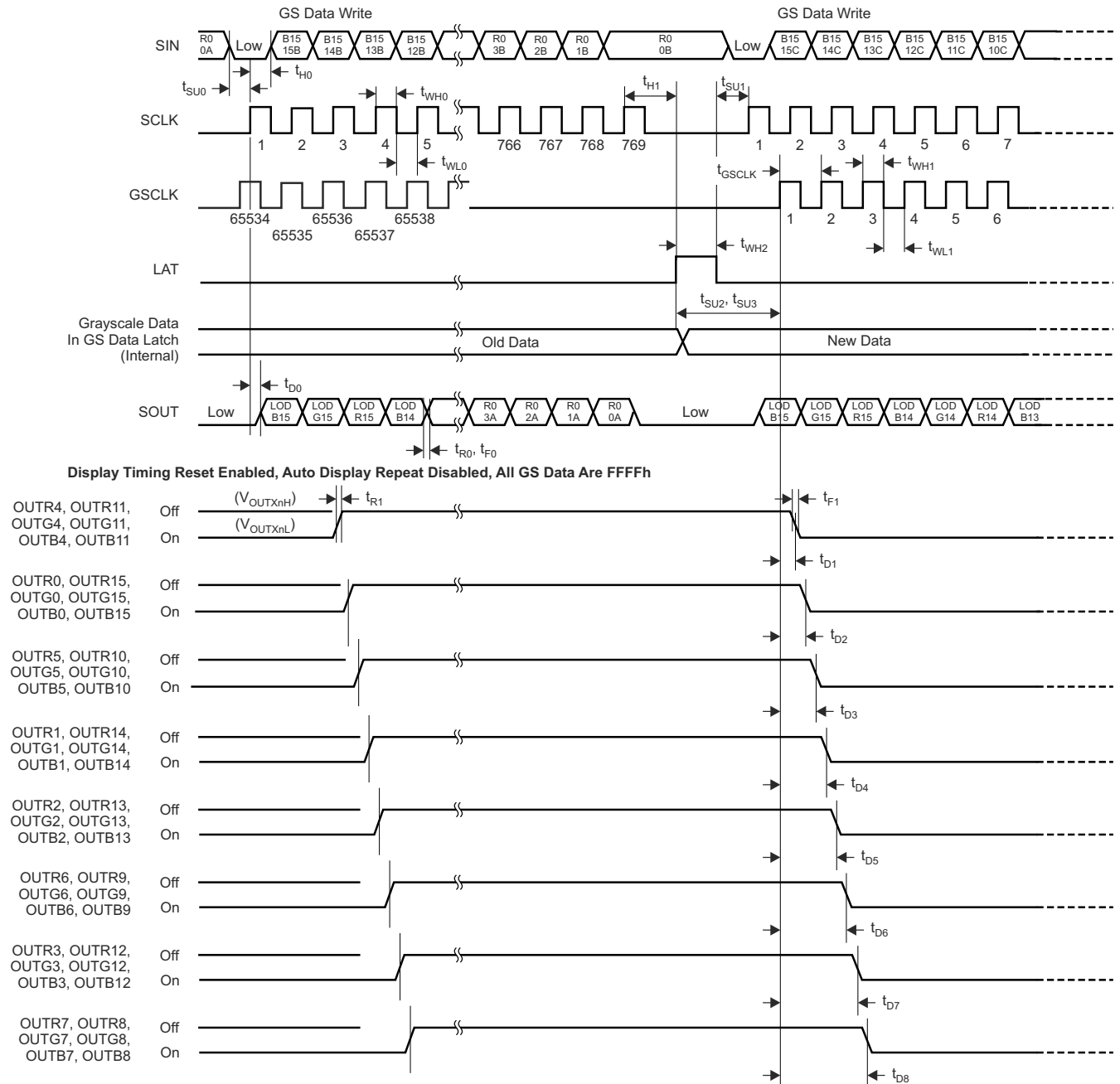
图 7-9. Data Input, Output, and Constant Output Timing
