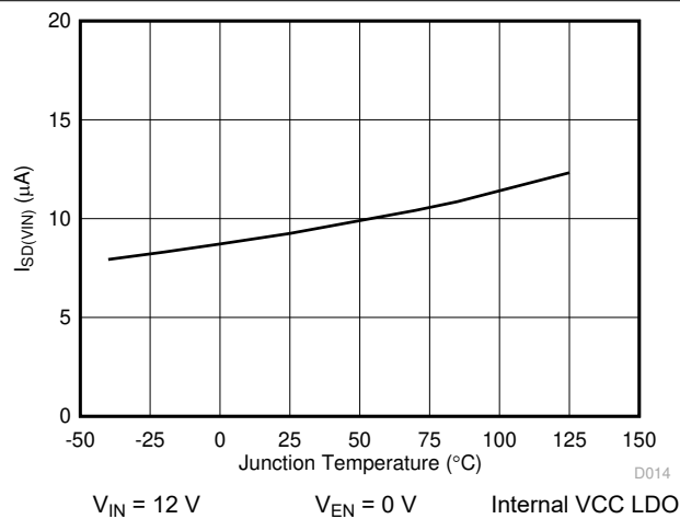
图 6-11. I_{SD(VIN)} vs Junction Temperature
