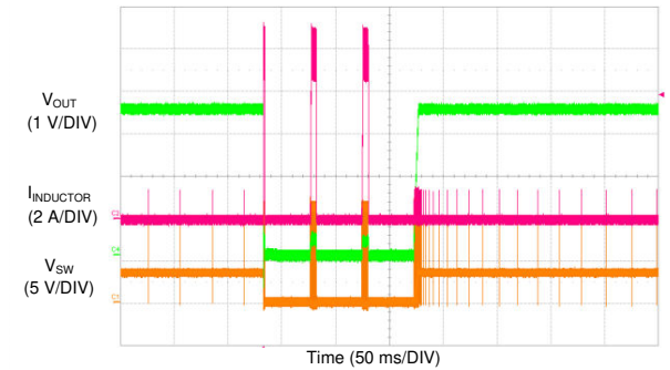
图 8-22. TPS7H4010-SEP Switching Waveform at Dropout
