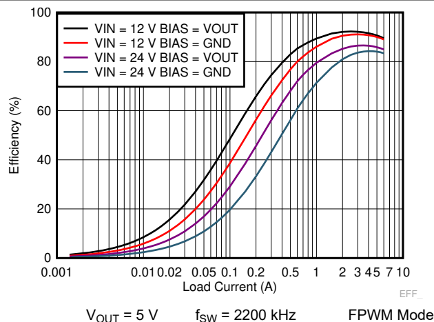
图 7-7. TPS7H4010 Efficiency Comparison With Bias = V_{OUT} to Bias = GND in FPWM Mode
