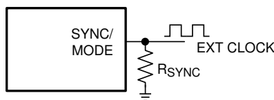
图 7-13. Frequency Synchronization
