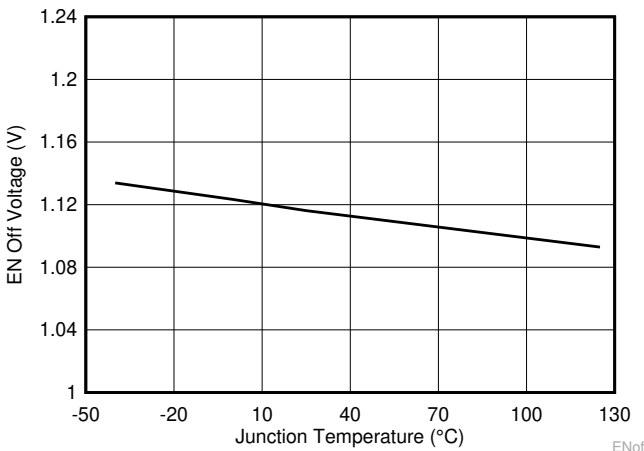
图 6-5. Enable Off Voltage vs Junction Temperature
