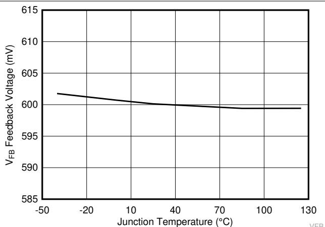
图 6-3. Feedback Voltage vs Junction Temperature
