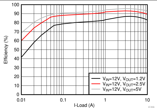
图 6-18. Efficiency vs Load Current, F_{SW} = 800 \text{ kHz} , OOA
