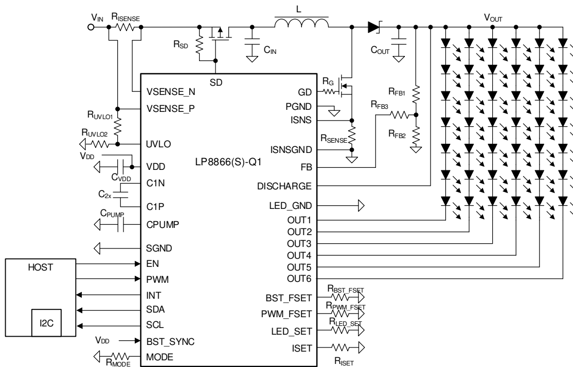
图 8-1. Full Feature Application for Display Backlight
