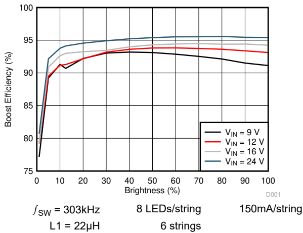
图 5-2. Boost Efficiency
