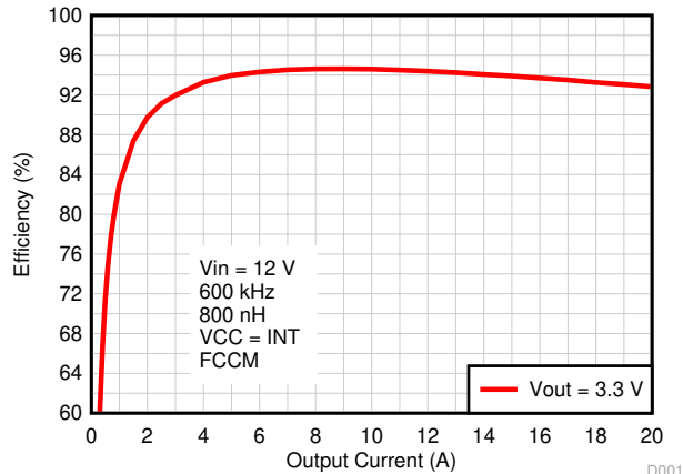
Figure 8-2. Efficiency vs Output Current, Internal VCC Bias
