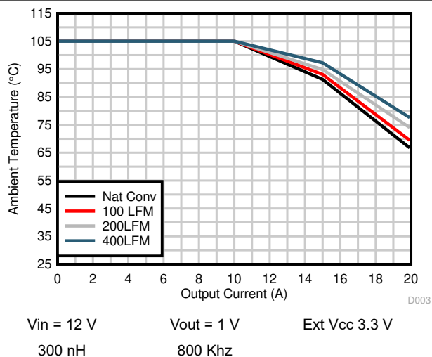
Figure 6-5. Safe Operating Area, V_{OUT} = 1 V
