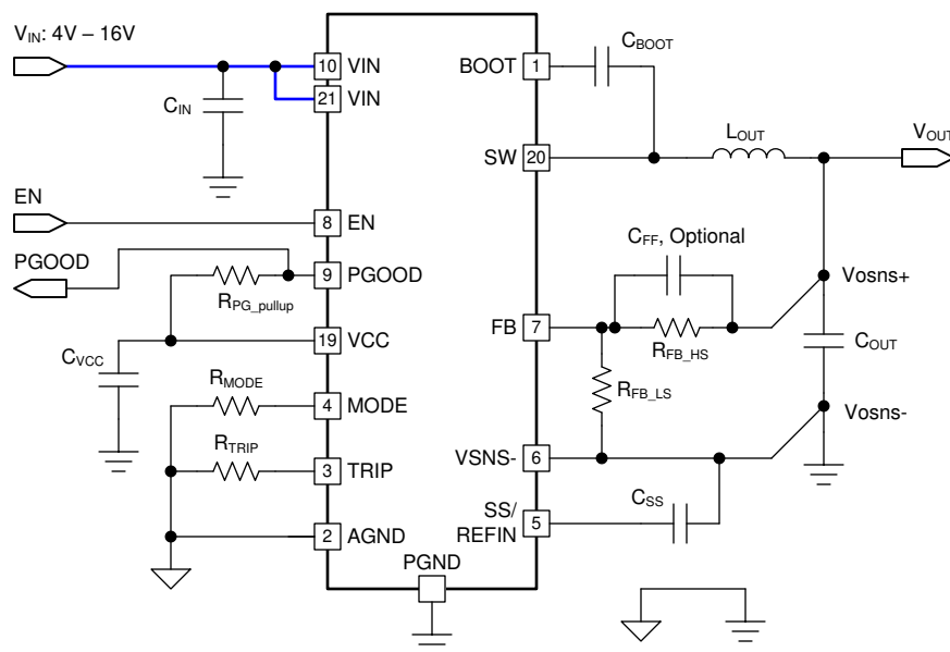
Figure 7-3. Single VIN Configuration For 12-V Bus
