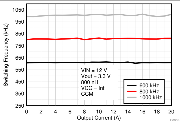
Figure 8-6. Switching Frequency vs Output Current
