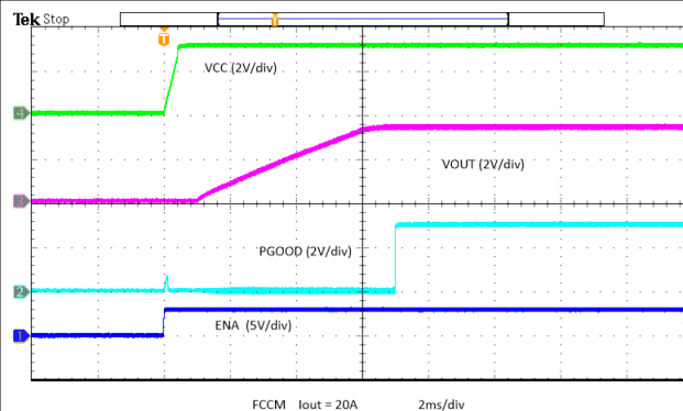
Figure 8-15. Enable Start-Up, Full Load
