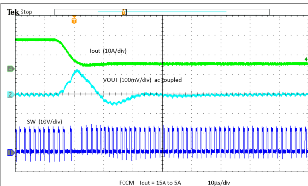
Figure 6-13. FCCM Mode Load Transient
