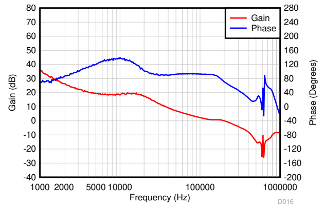
Figure 6-20. Frequency Response, 20 A Load
