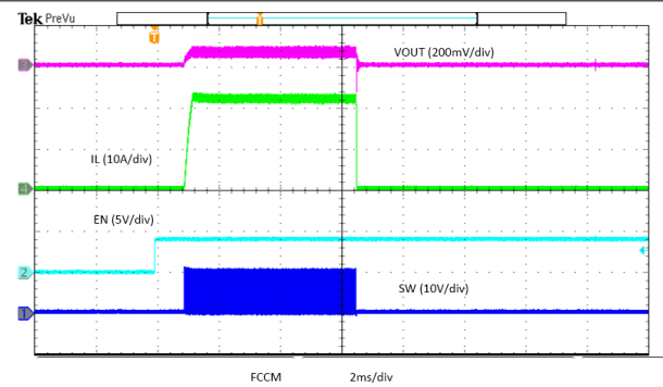
Figure 6-22. Enable into Overcurrent
