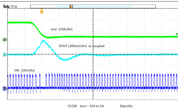
Figure 8-26. Unload Transient
