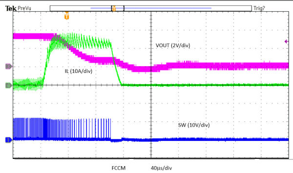
Figure 6-21. Overcurrent Protection
