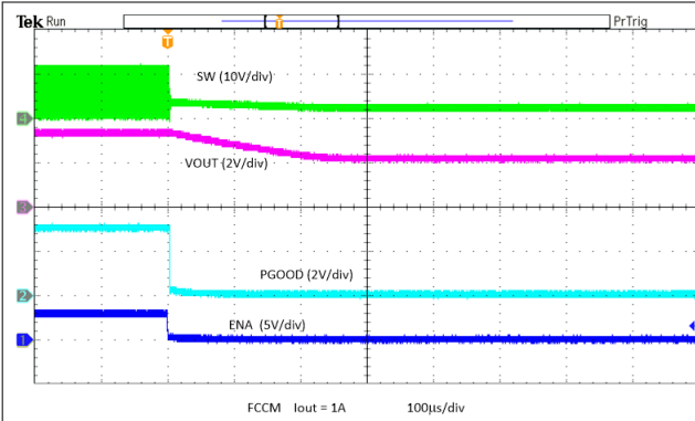
Figure 8-20. Prebias Power-Down
