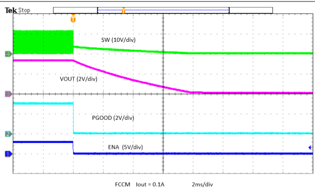
Figure 8-18. Enable Power Down Iout = 0.1 A
