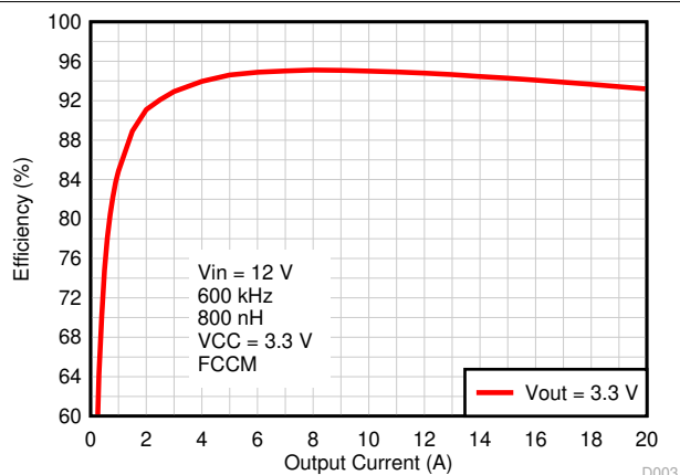
Figure 8-4. Efficiency vs Output Current, VCC = 3.3V External VCC Bias
