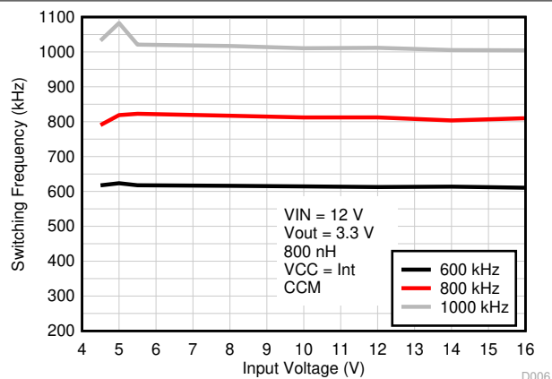
Figure 8-7. Switching Frequency vs Input Voltage
