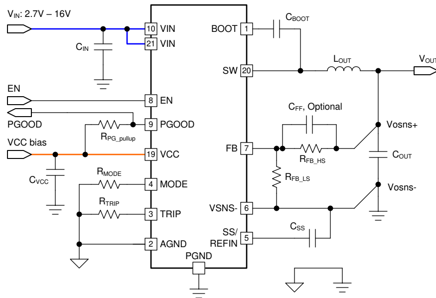
Figure 7-5. Split Rail Configuration With External VCC Bias
