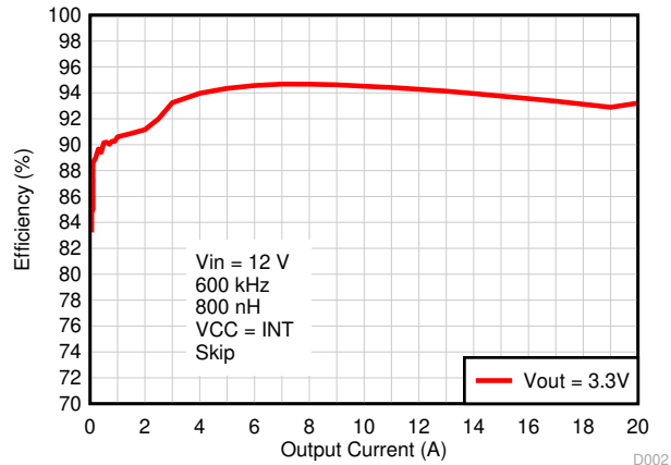
Figure 8-3. Efficiency vs Output Current, Internal VCC Bias
