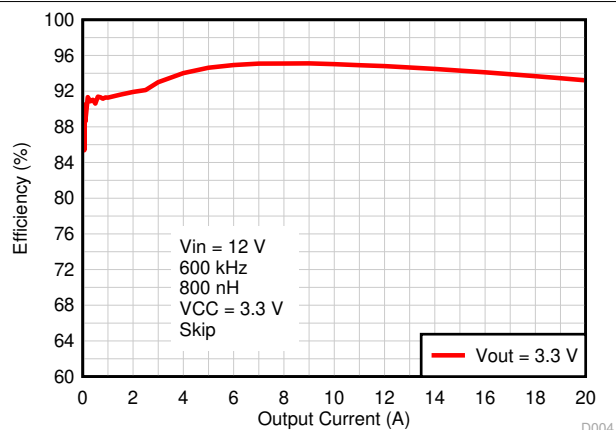
Figure 8-5. Efficiency vs Output Current, VCC = 3.3V External VCC Bias
