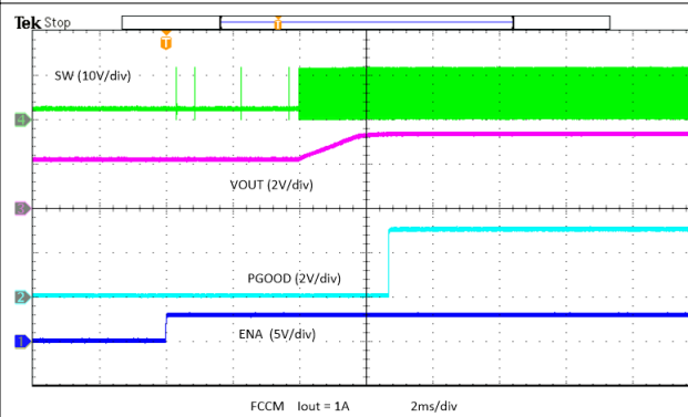
Figure 8-19. Enable Start-Up, Prebias
