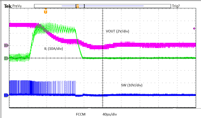
Figure 8-33. Overcurrent Protection
