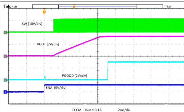
Figure 8-17. Enable to Power Up Iout = 0.1 A
