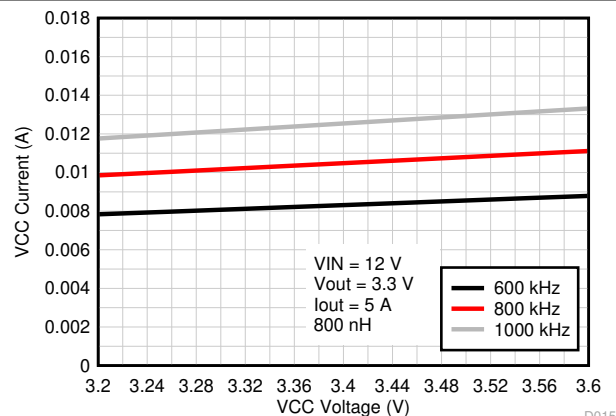
Figure 8-14. ICC Current vs External VCC Voltage
