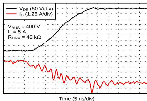
图 6. Turn-off Waveform in Application Example
