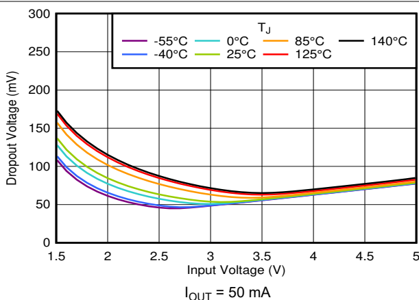
图 6-36. Dropout vs V_{IN} and Temperature
