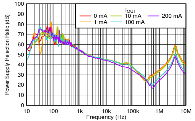
V_{IN} = 2.8\text{ V} , V_{OUT} = 1.8\text{ V} , C_{OUT} = 1\text{ }\mu\text{F} 图 6-44. PSRR vs Frequency and I_{OUT}
