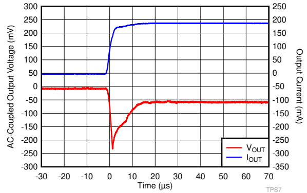
图 6-20. I_{OUT} Transient From 0 mA to 200 mA
