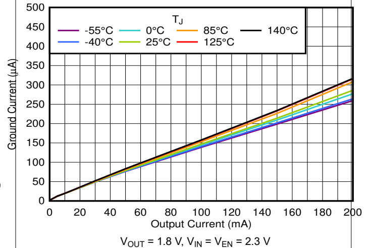
图 6-4. I_Q vs I_{OUT} and Temperature Up to 200 mA
