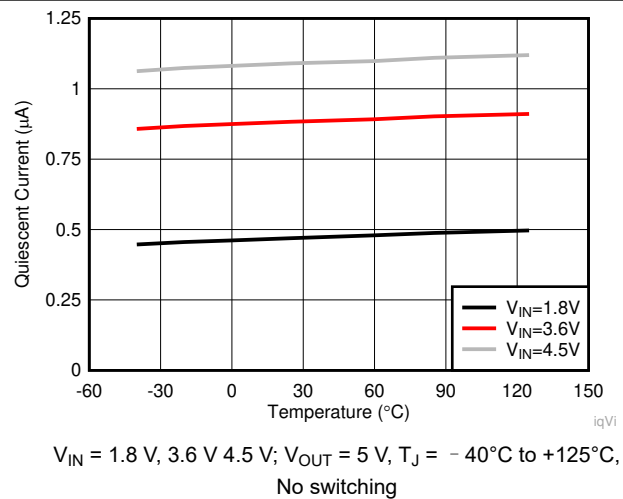
图 6-6. Quiescent Current into VIN vs Temperature
