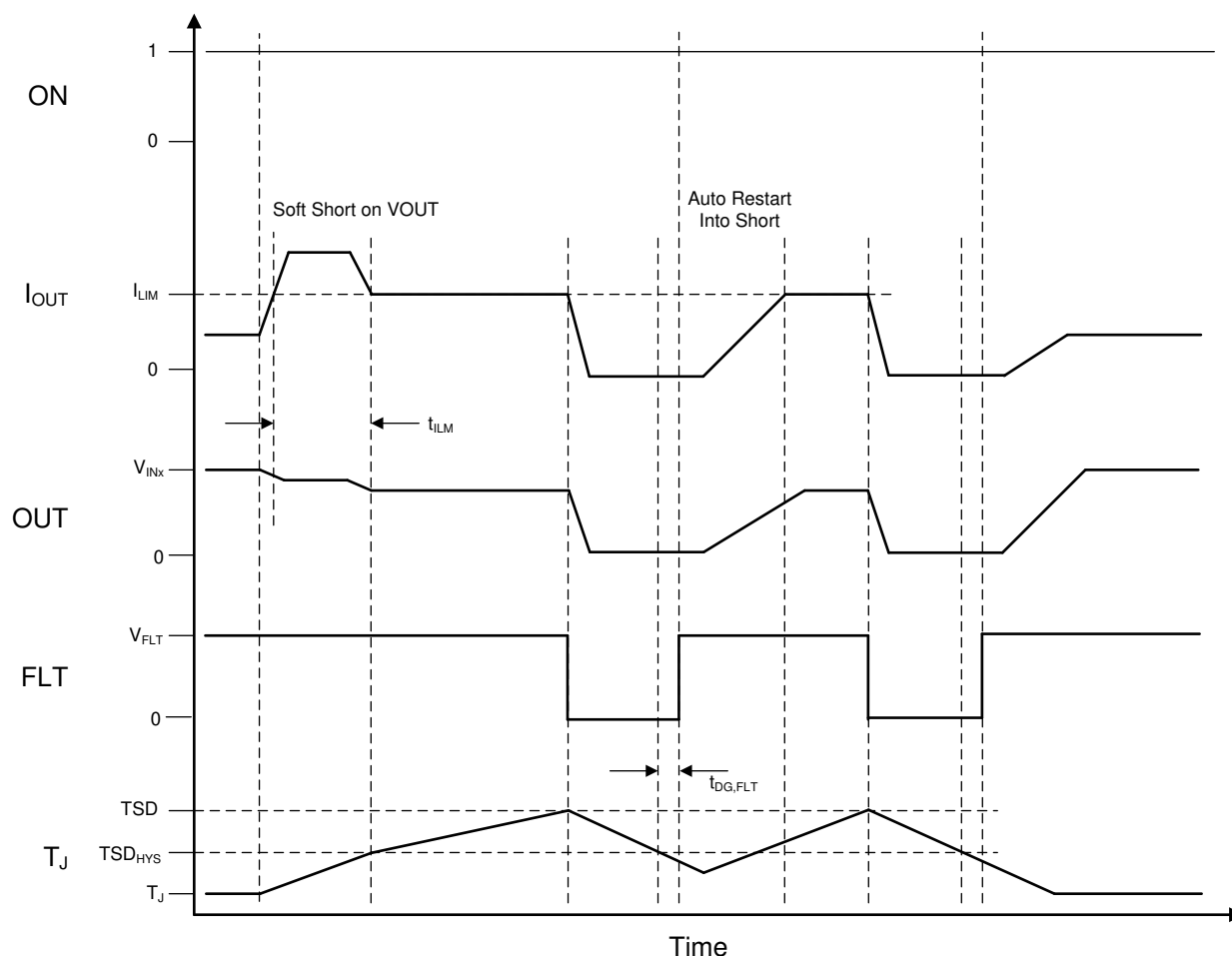
图 6. TPS22948 Current Limiting Behavior
