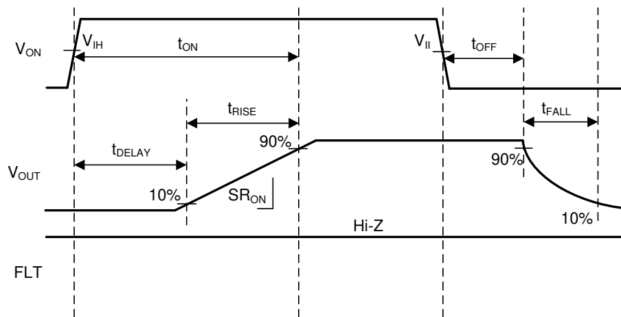
图 5. Timing Waveforms
