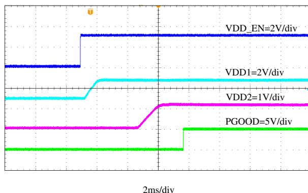
图 8-14. Start-Up Through VDD_EN, I_{VDD1OUT} = 0\text{ A} , I_{VDD2OUT} = 0\text{ A}
