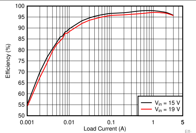
图 12. V_{OUT}=3.3\text{ V} Efficiency, L=4.7\text{ }\mu\text{H}
