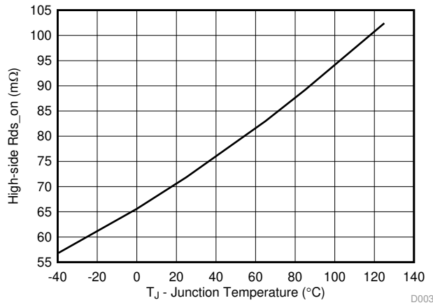
图 3. High-side R_{ds-On} VS Junction Temperature
