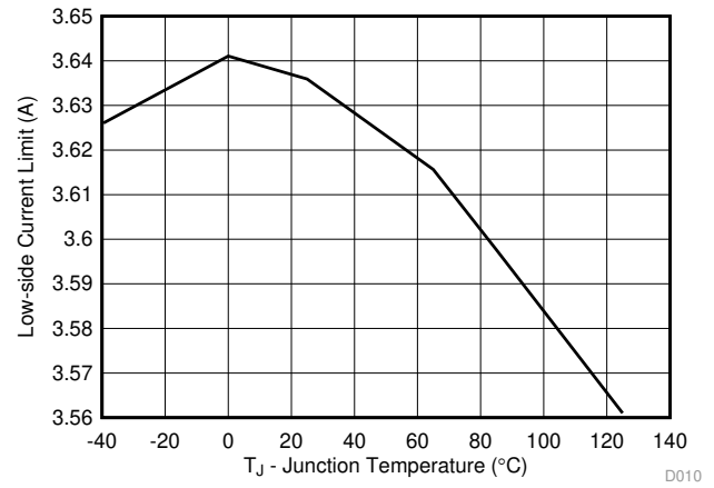
图 10. Low-side Current Limit Threshold VS Junction Temperature
