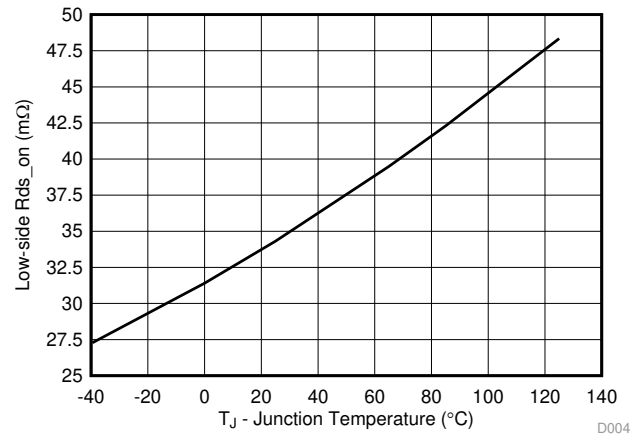
图 4. Low-side R_{ds-On} VS Junction Temperature
