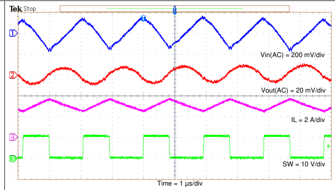
图 25. Steady State Waveforms, I_{OUT} = 3\text{ A}
