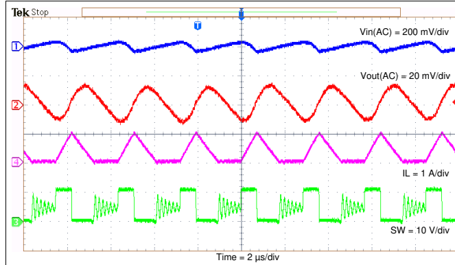
图 24. Steady State Waveforms, I_{OUT} = 0.3\text{ A}
