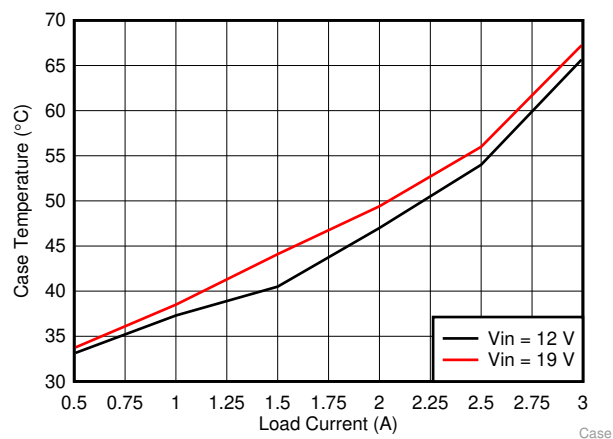
图 22. Case Temperature Rise vs Load Current
